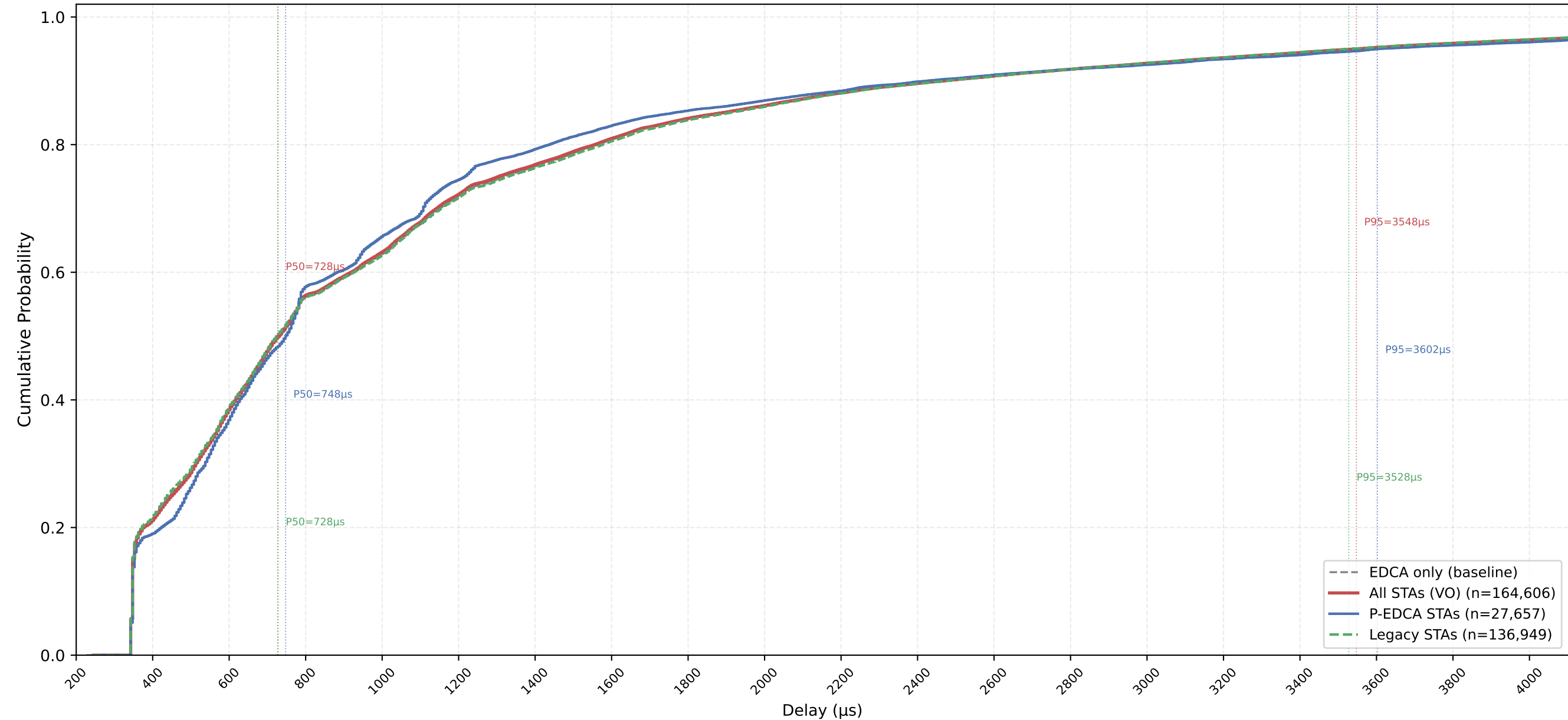
VO Delay CDF — P-EDCA / Legacy / All | CWds=0 × QSRC=4 × PSRC=1 nSta=30, nPedca=5/30, 0.5Mbps, avg of 10 runs
