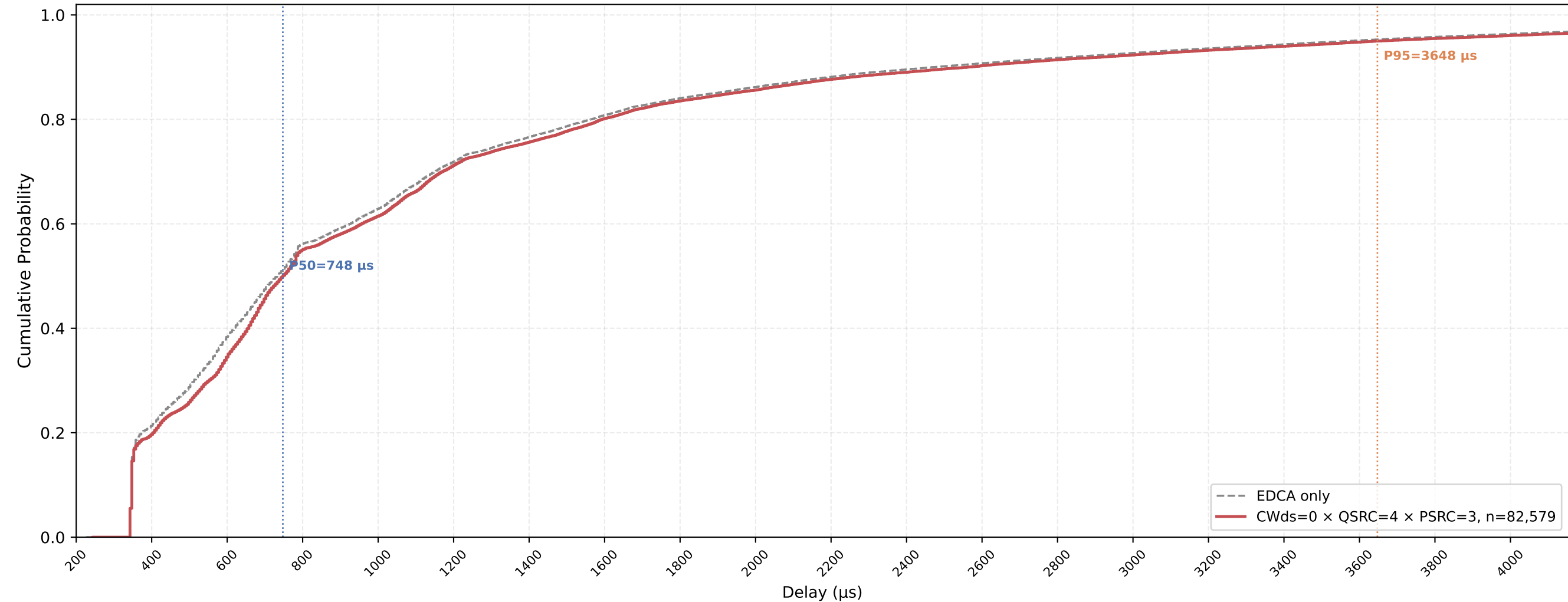
Legacy STA VO Delay CDF — CWds=0 × QSRC=4 × PSRC=3 nSta=30, nPedca=15, 0.5Mbps, avg of 10 runs
