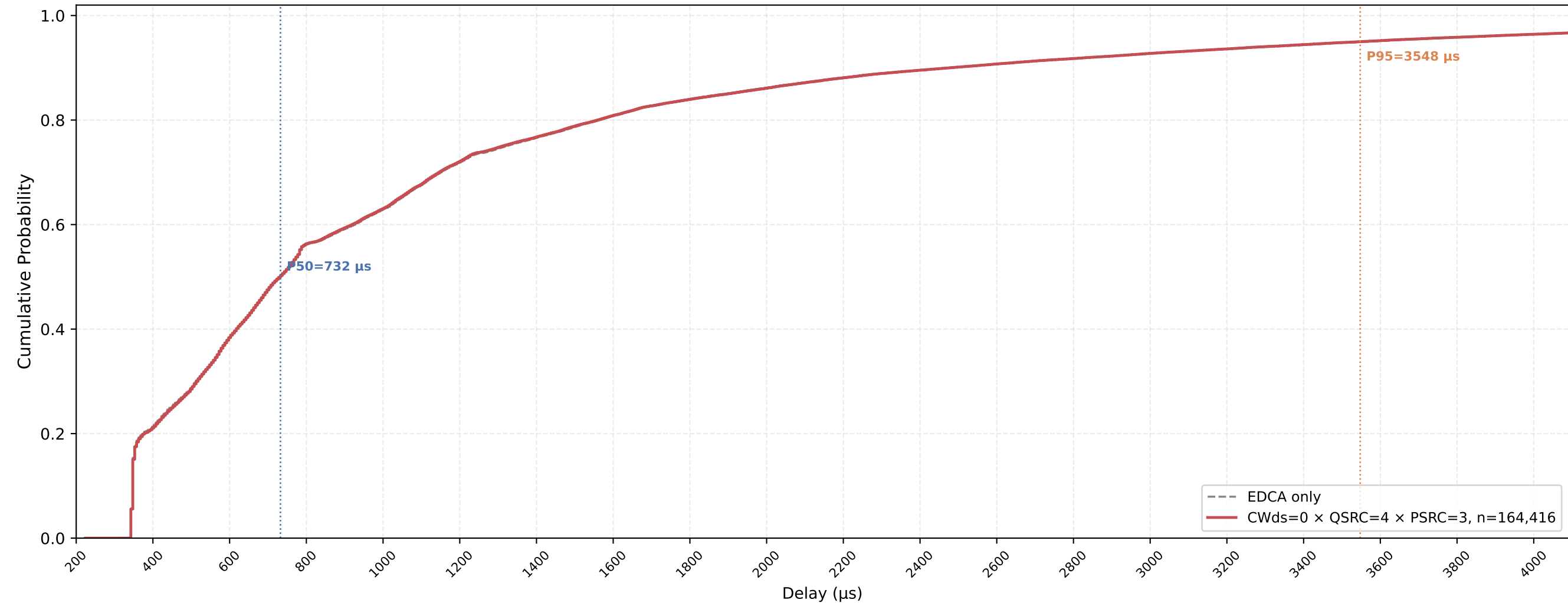
VO (all STAs) Delay CDF — CWds=0 × QSRC=4 × PSRC=3 nSta=30, nPedca=5, 0.5Mbps, avg of 10 runs
