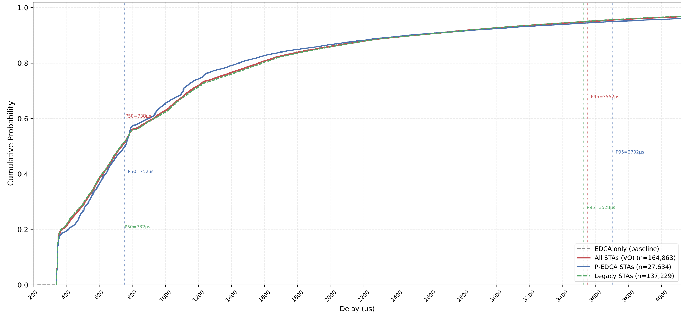
VO Delay CDF — P-EDCA / Legacy / All | CWds=0 × QSRC=5 × PSRC=1 nSta=30, nPedca=5/30, 0.5Mbps, avg of 10 runs
