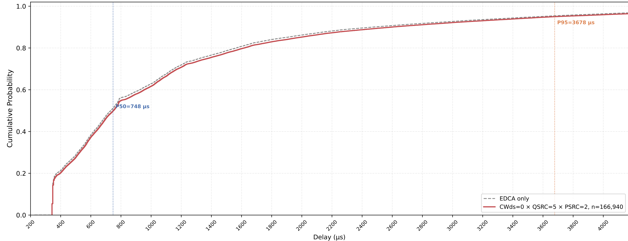
P-EDCA STA VO Delay CDF — CWds=0 × QSRC=5 × PSRC=2 nSta=30, nPedca=30, 0.5Mbps, avg of 10 runs
