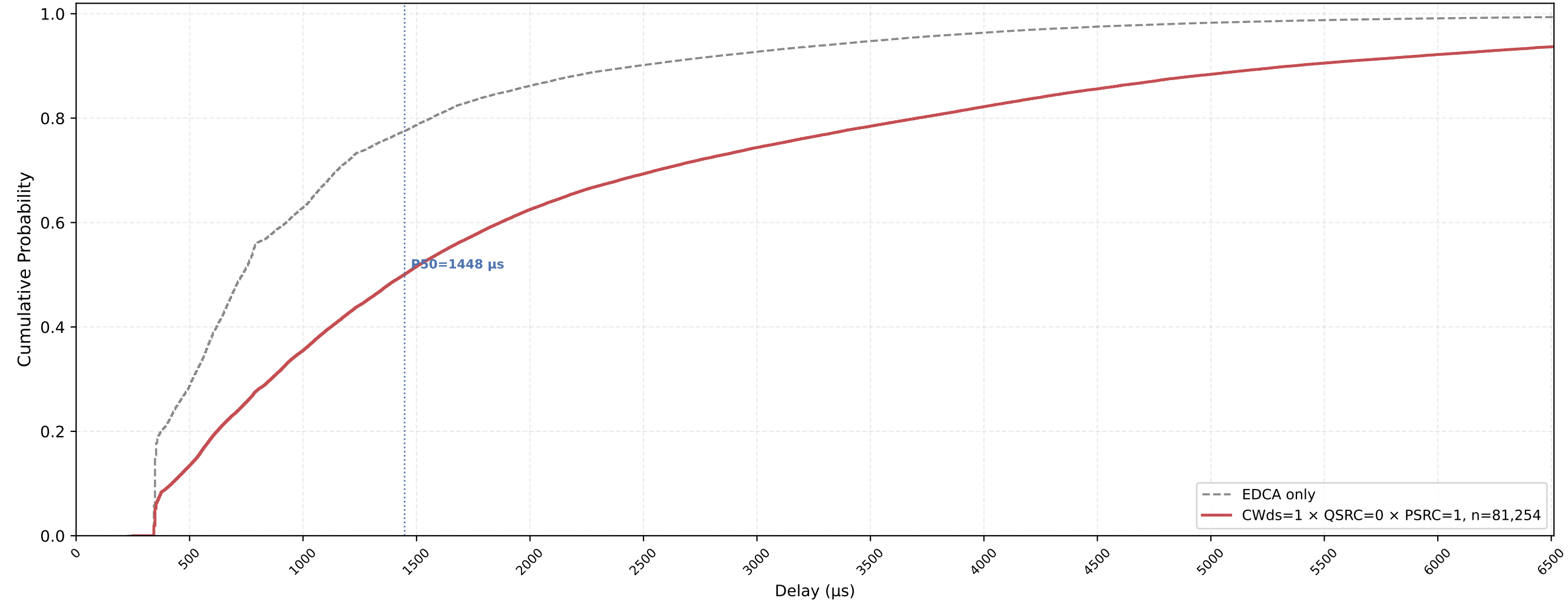
Legacy STA VO Delay CDF — CWds=1 × QSRC=0 × PSRC=1 nSta=30, nPedca=15, 0.5Mbps, avg of 10 runs
