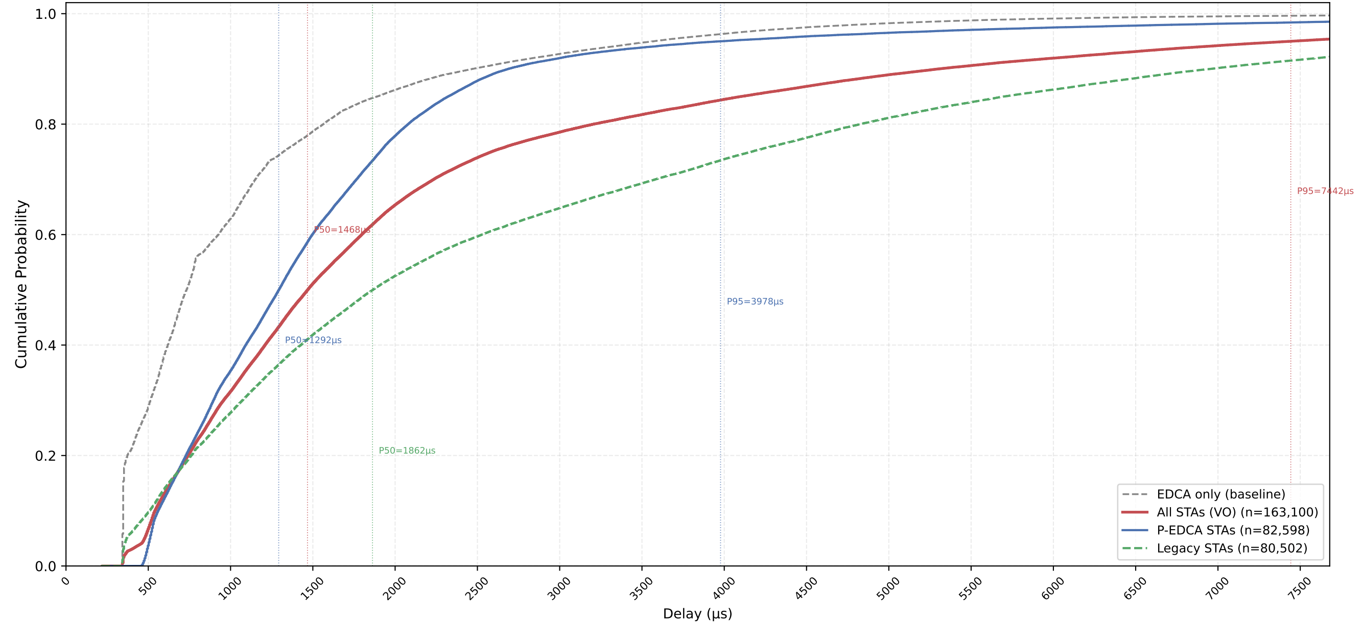
VO Delay CDF — P-EDCA / Legacy / All | CWds=1 × QSRC=0 × PSRC=2 nSta=30, nPedca=15/30, 0.5Mbps, avg of 10 runs
