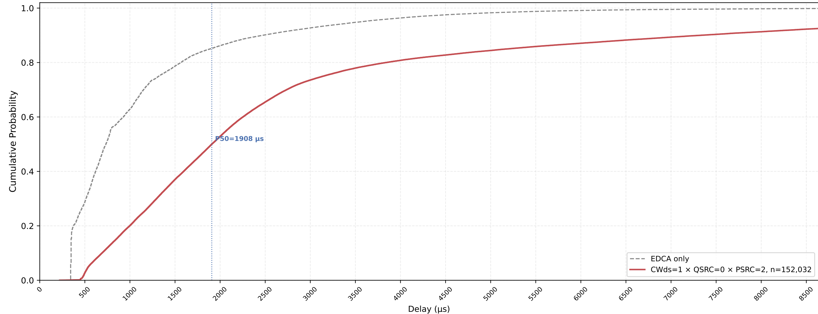
VO (all STAs) Delay CDF — CWds=1 × QSRC=0 × PSRC=2 nSta=30, nPedca=30, 0.5Mbps, avg of 10 runs
