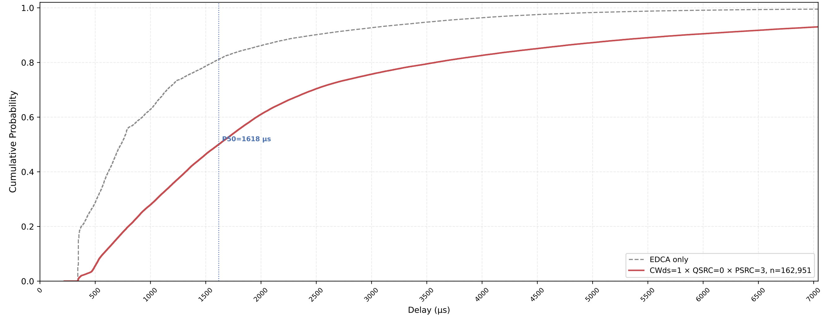
VO (all STAs) Delay CDF — CWds=1 × QSRC=0 × PSRC=3 nSta=30, nPedca=15, 0.5Mbps, avg of 10 runs
