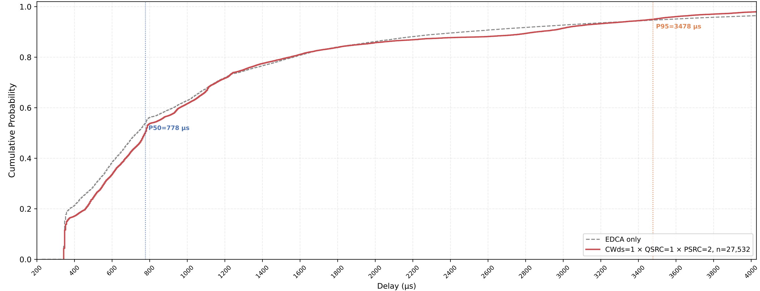
P-EDCA STA VO Delay CDF — CWds=1 × QSRC=1 × PSRC=2 nSta=30, nPedca=5, 0.5Mbps, avg of 10 runs
