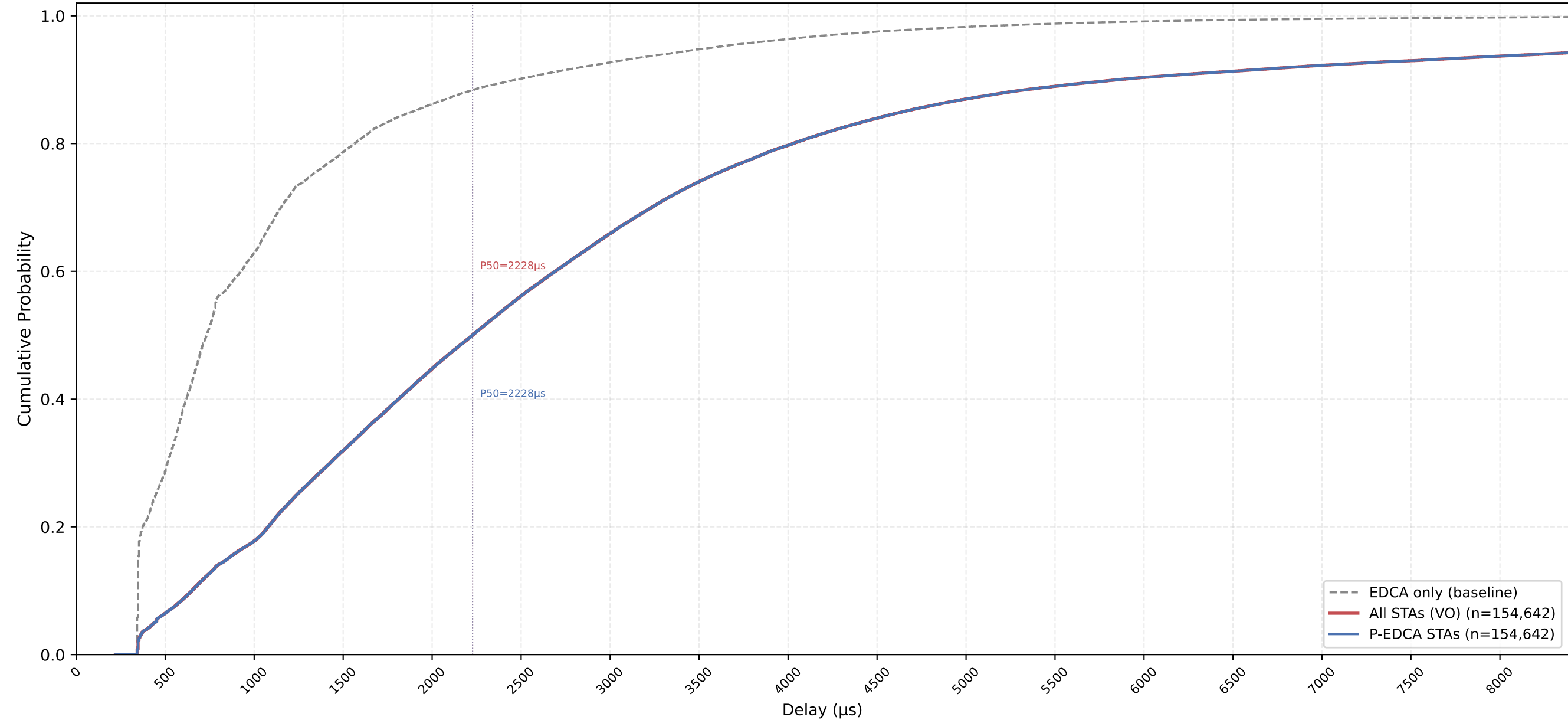
VO Delay CDF — P-EDCA / Legacy / All | CWds=1 × QSRC=1 × PSRC=3 nSta=30, nPedca=30/30, 0.5Mbps, avg of 10 runs
