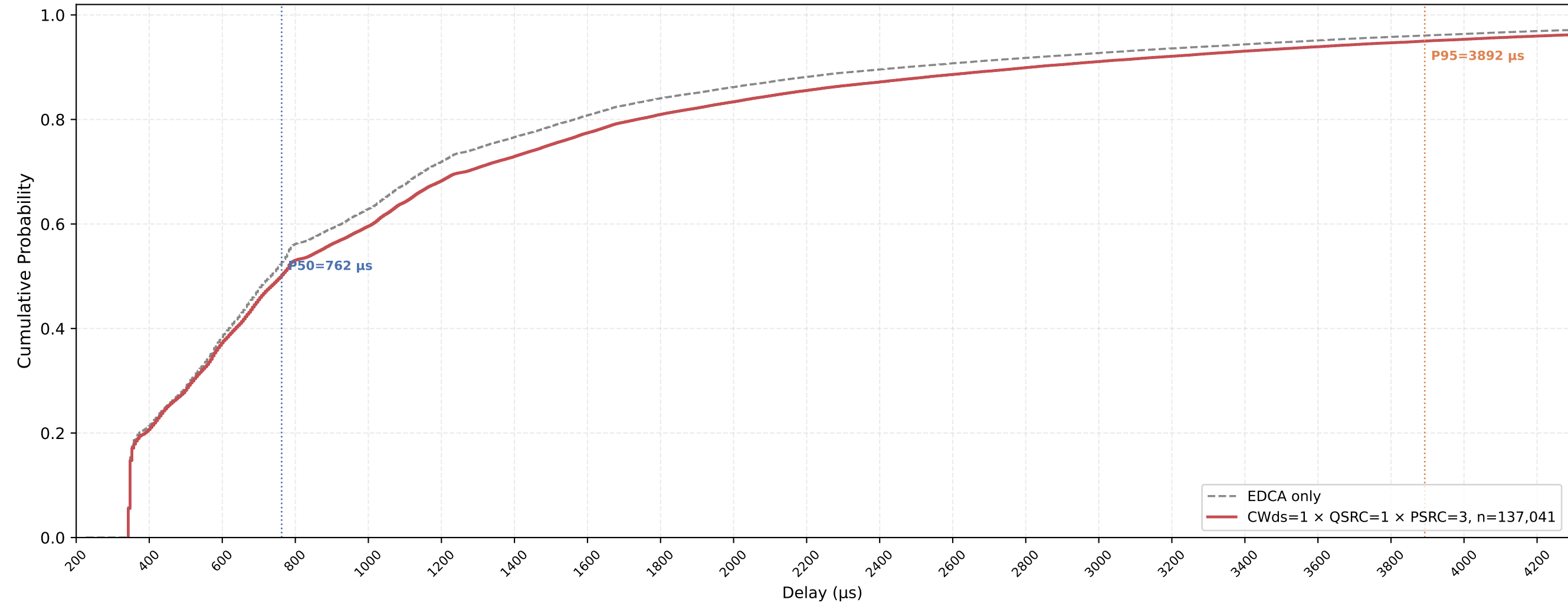
Legacy STA VO Delay CDF — CWds=1 × QSRC=1 × PSRC=3 nSta=30, nPedca=5, 0.5Mbps, avg of 10 runs
