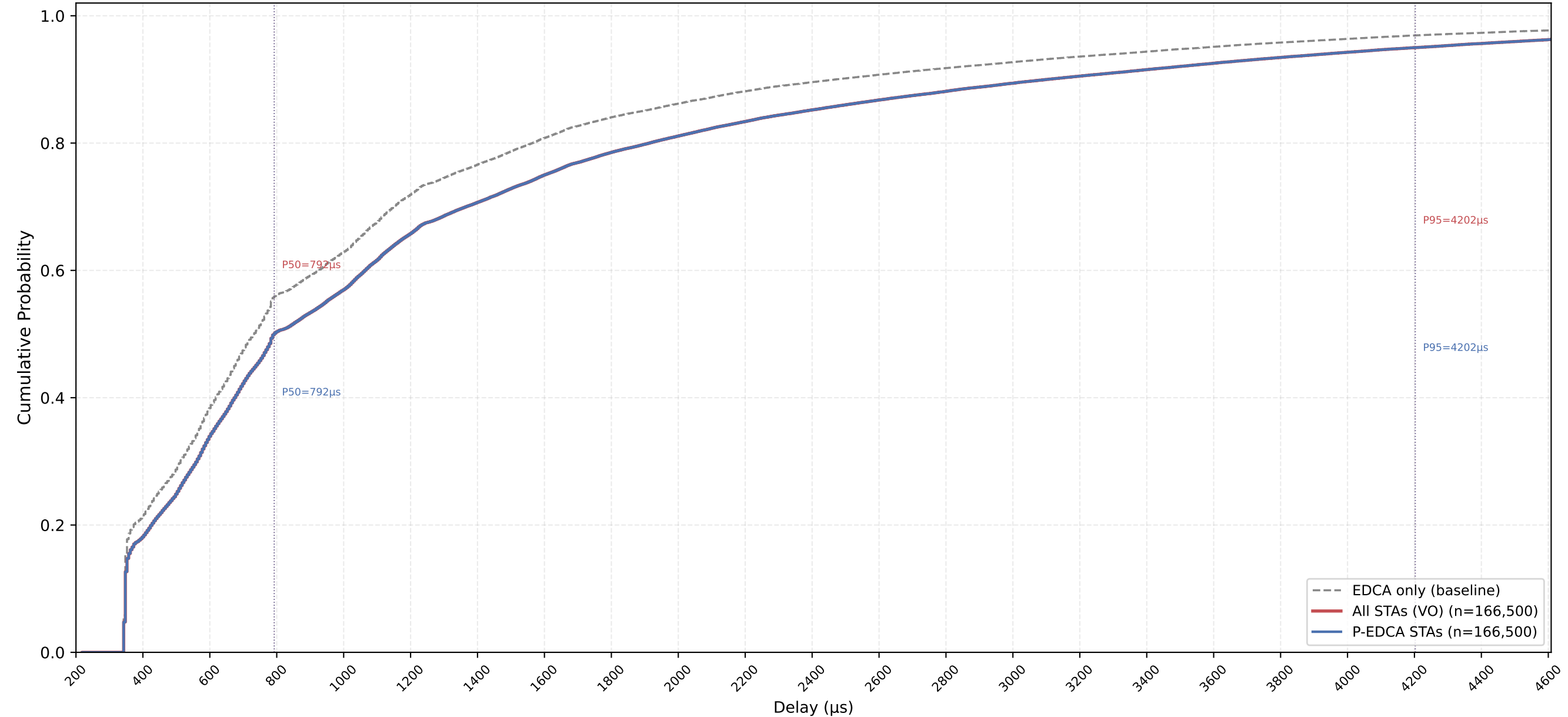
VO Delay CDF — P-EDCA / Legacy / All | CWds=1 × QSRC=2 × PSRC=1 nSta=30, nPedca=30/30, 0.5Mbps, avg of 10 runs
