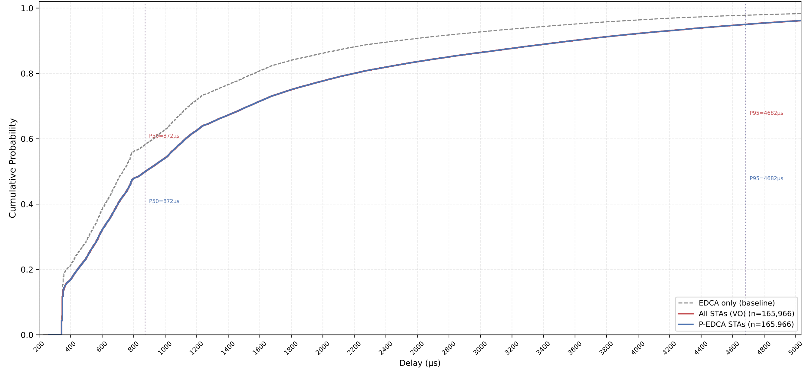
VO Delay CDF — P-EDCA / Legacy / All | CWds=1 × QSRC=2 × PSRC=2 nSta=30, nPedca=30/30, 0.5Mbps, avg of 10 runs
