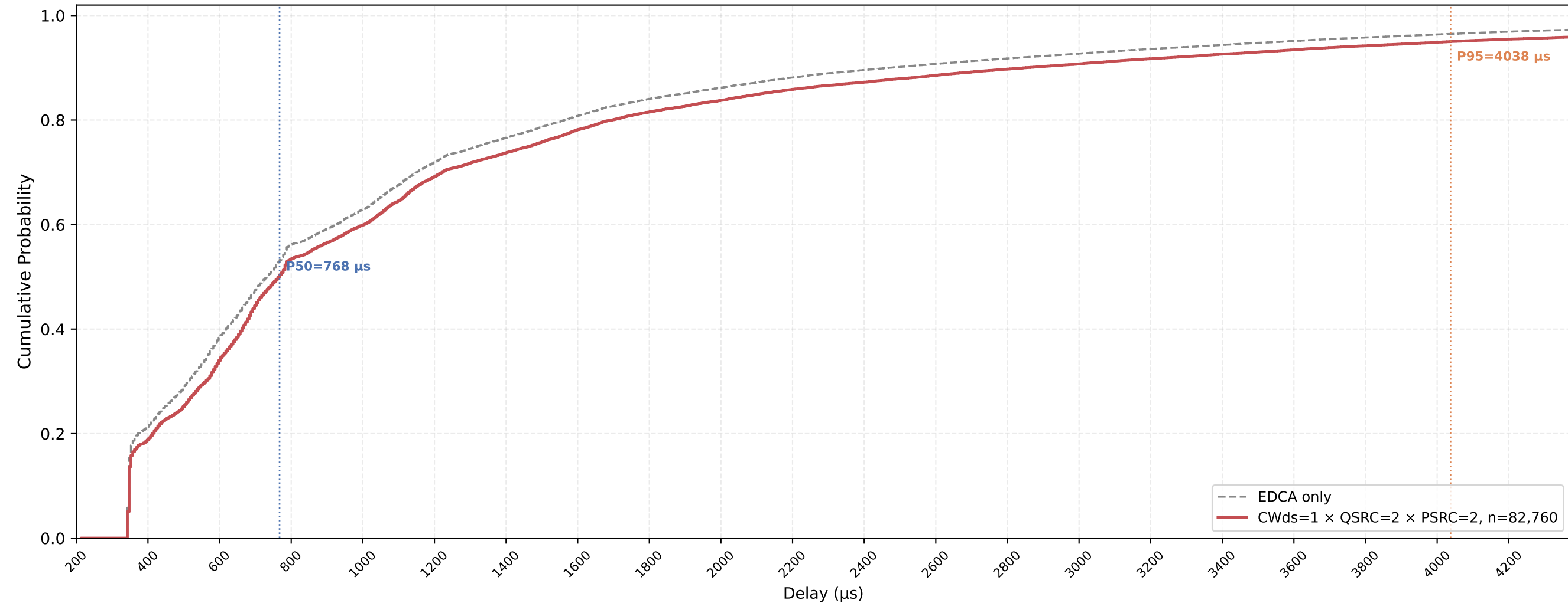
Legacy STA VO Delay CDF — CWds=1 × QSRC=2 × PSRC=2 nSta=30, nPedca=15, 0.5Mbps, avg of 10 runs
