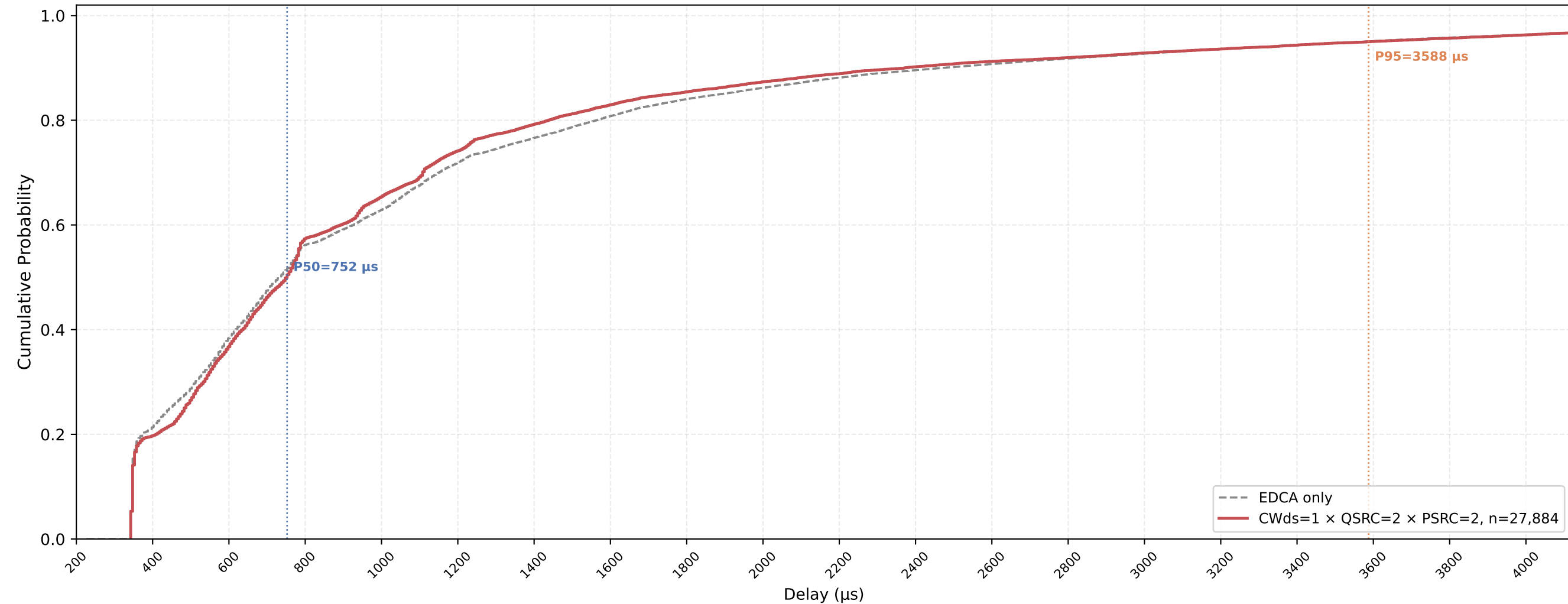
P-EDCA STA VO Delay CDF — CWds=1 × QSRC=2 × PSRC=2 nSta=30, nPedca=5, 0.5Mbps, avg of 10 runs
