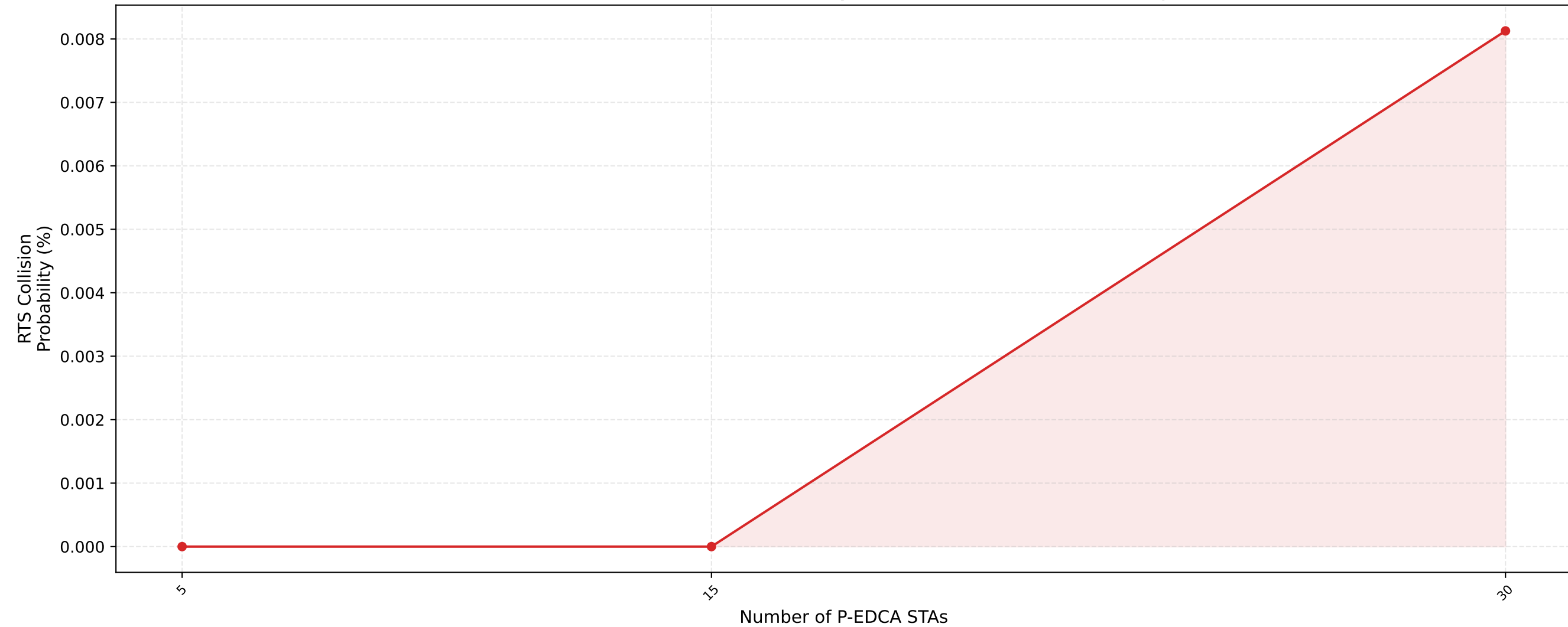
[Stat 6] P-EDCA RTS Collision Probability — nSta=30, 0.5Mbps (avg of 10 runs)
