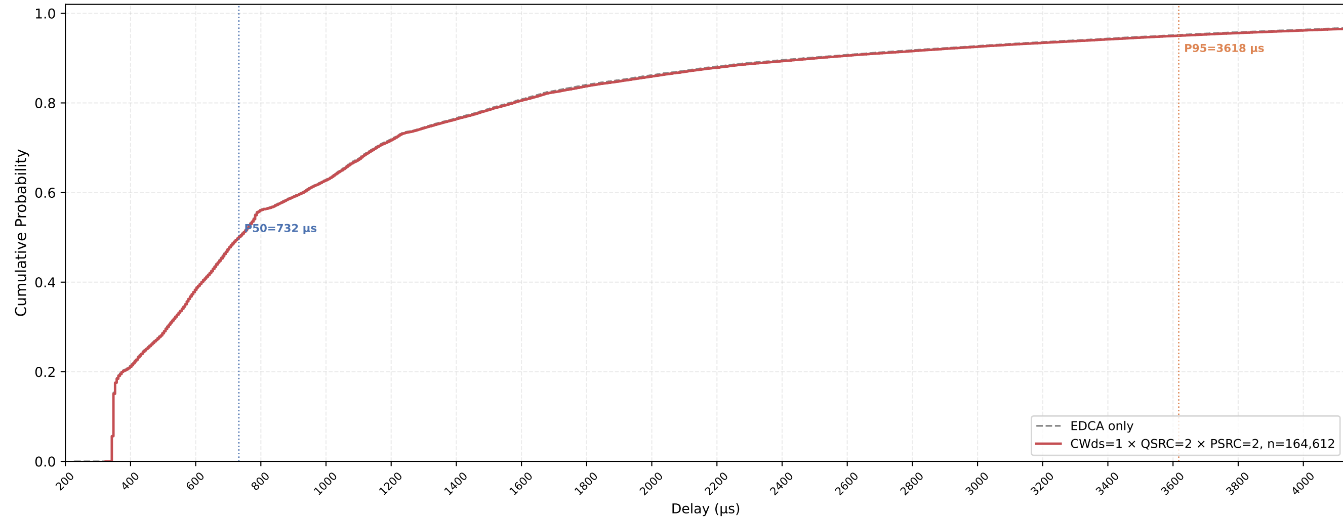
VO (all STAs) Delay CDF — CWds=1 × QSRC=2 × PSRC=2 nSta=30, nPedca=5, 0.5Mbps, avg of 10 runs
