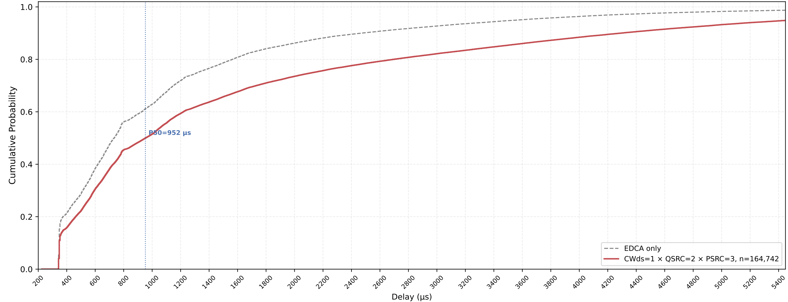
P-EDCA STA VO Delay CDF — CWds=1 × QSRC=2 × PSRC=3 nSta=30, nPedca=30, 0.5Mbps, avg of 10 runs
