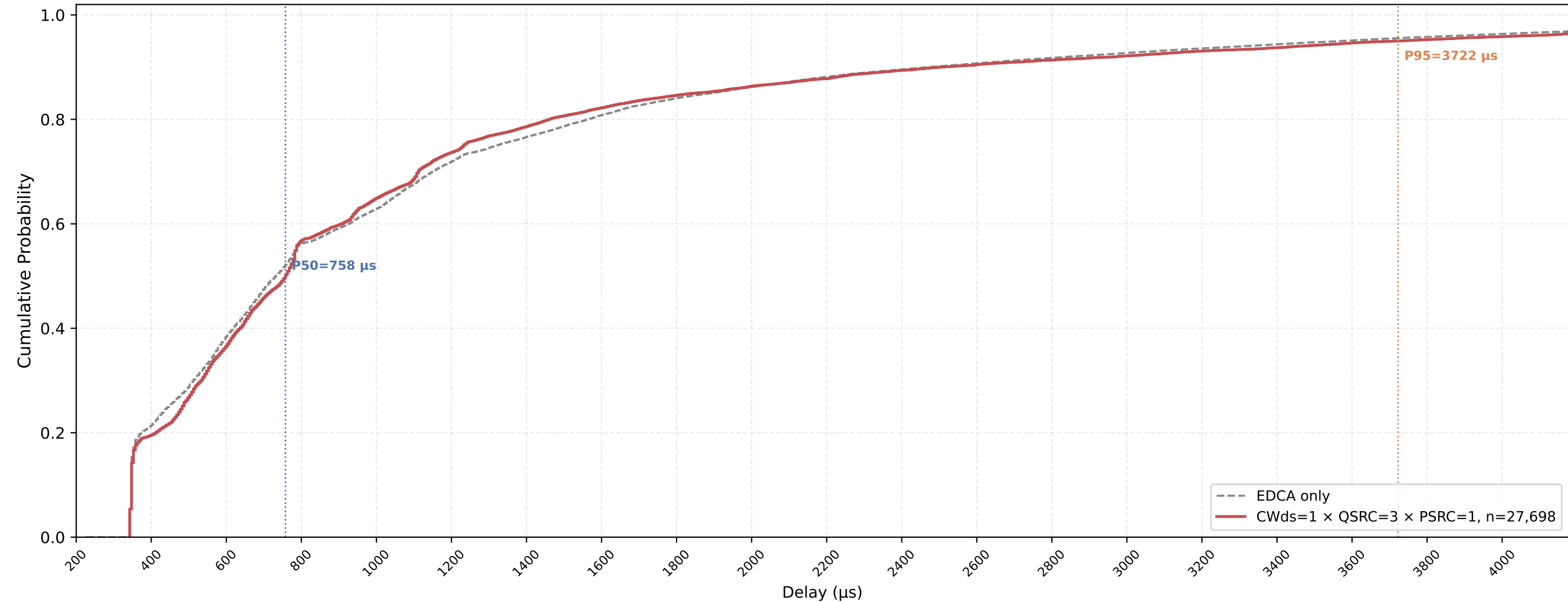
P-EDCA STA VO Delay CDF — CWds=1 × QSRC=3 × PSRC=1 nSta=30, nPedca=5, 0.5Mbps, avg of 10 runs
