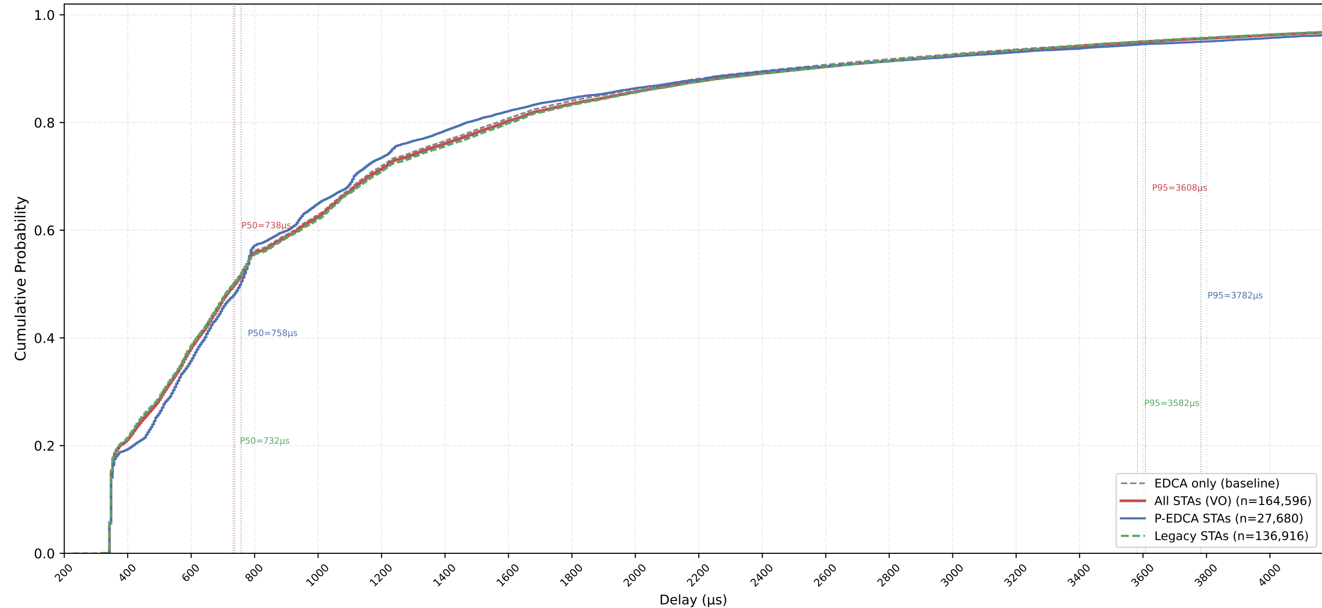
VO Delay CDF — P-EDCA / Legacy / All | CWds=1 × QSRC=3 × PSRC=3 nSta=30, nPedca=5/30, 0.5Mbps, avg of 10 runs
