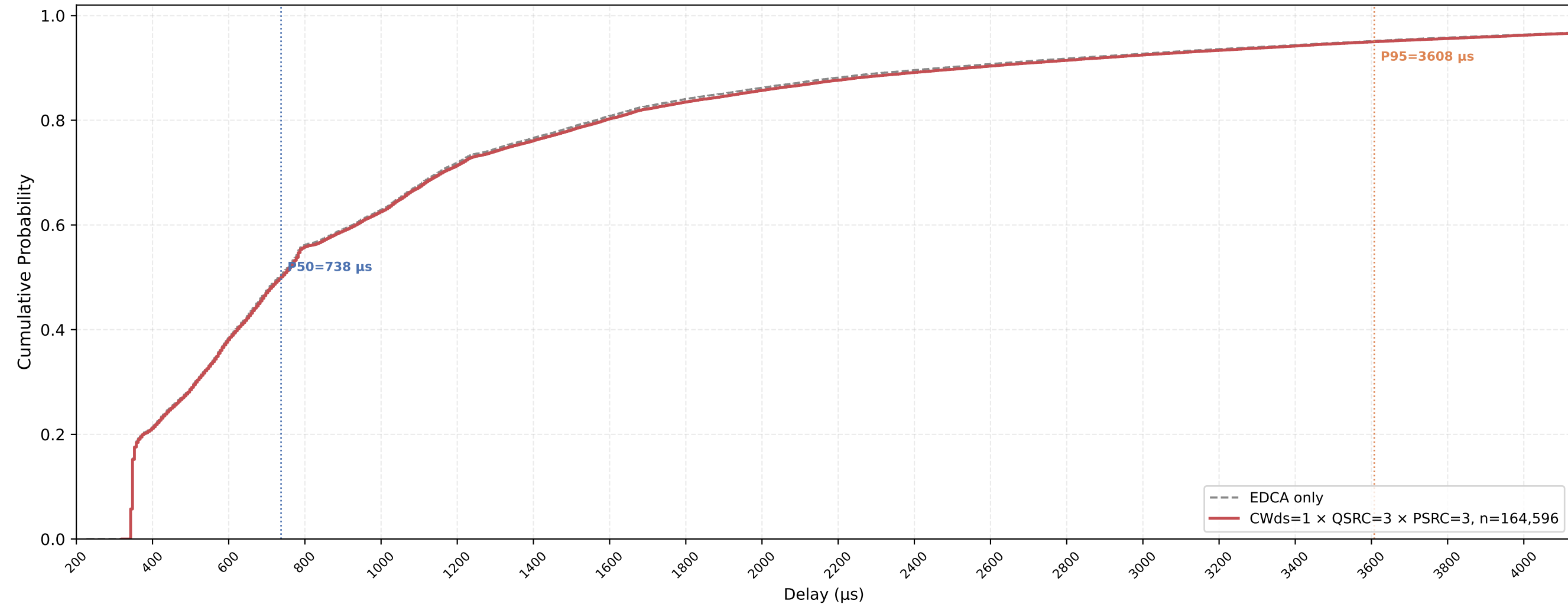
VO (all STAs) Delay CDF — CWds=1 × QSRC=3 × PSRC=3 nSta=30, nPedca=5, 0.5Mbps, avg of 10 runs
