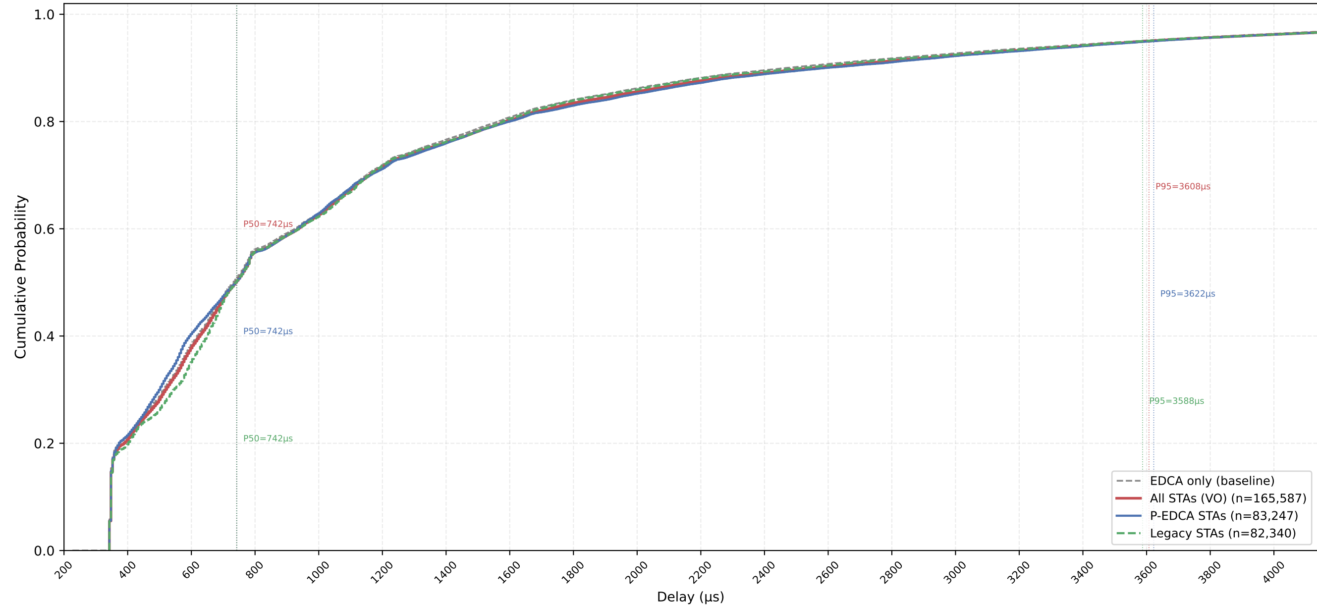
VO Delay CDF — P-EDCA / Legacy / All | CWds=1 × QSRC=4 × PSRC=2 nSta=30, nPedca=15/30, 0.5Mbps, avg of 10 runs
