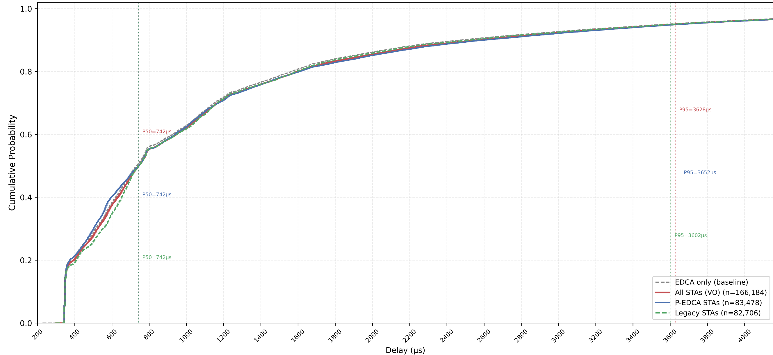
VO Delay CDF — P-EDCA / Legacy / All | CWds=1 × QSRC=4 × PSRC=3 nSta=30, nPedca=15/30, 0.5Mbps, avg of 10 runs
