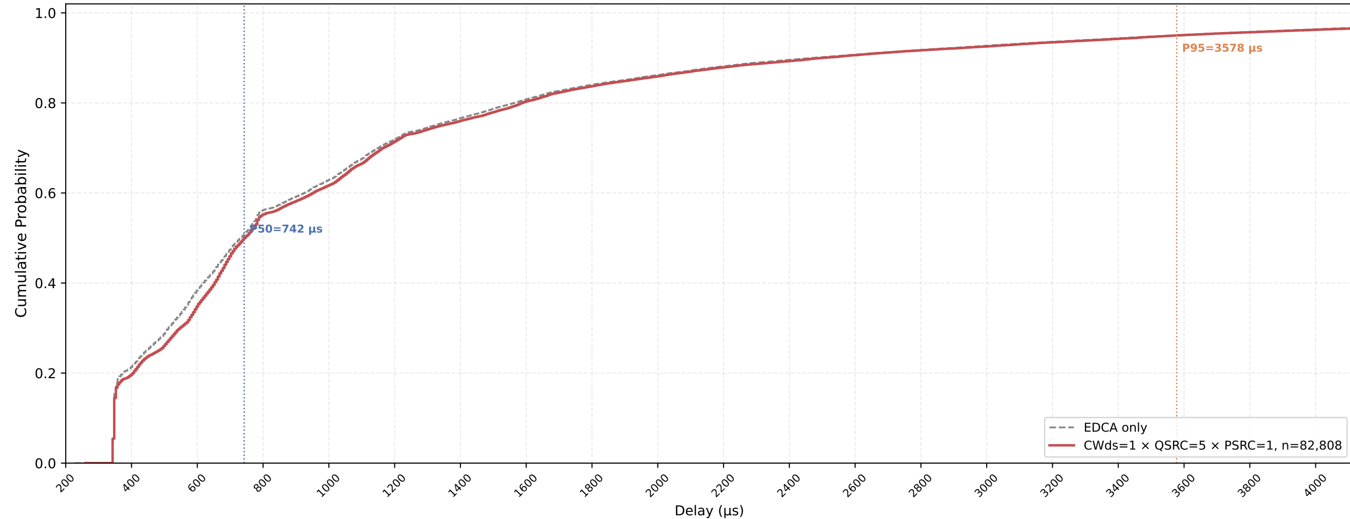
Legacy STA VO Delay CDF — CWds=1 × QSRC=5 × PSRC=1 nSta=30, nPedca=15, 0.5Mbps, avg of 10 runs
