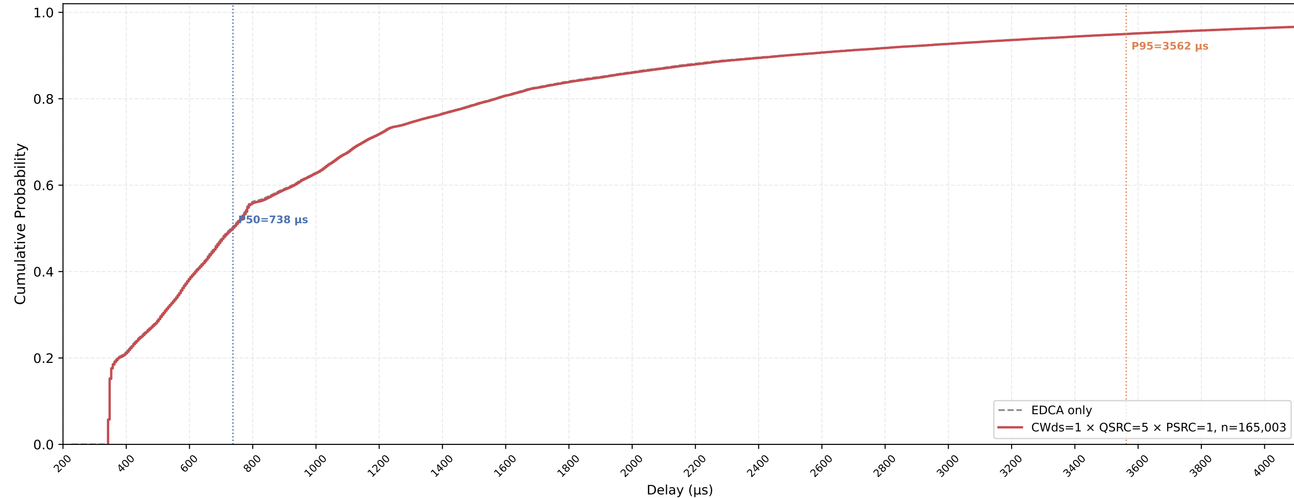
VO (all STAs) Delay CDF — CWds=1 × QSRC=5 × PSRC=1 nSta=30, nPedca=5, 0.5Mbps, avg of 10 runs
