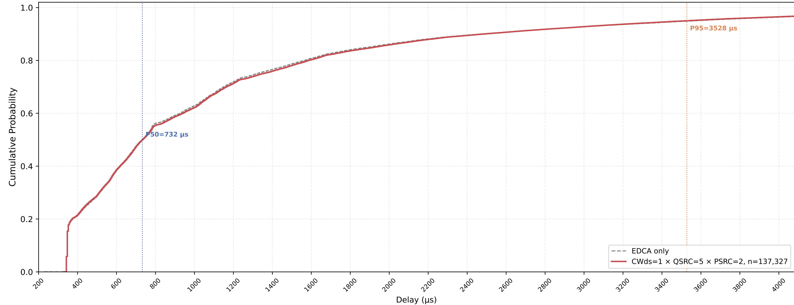
Legacy STA VO Delay CDF — CWds=1 × QSRC=5 × PSRC=2 nSta=30, nPedca=5, 0.5Mbps, avg of 10 runs
