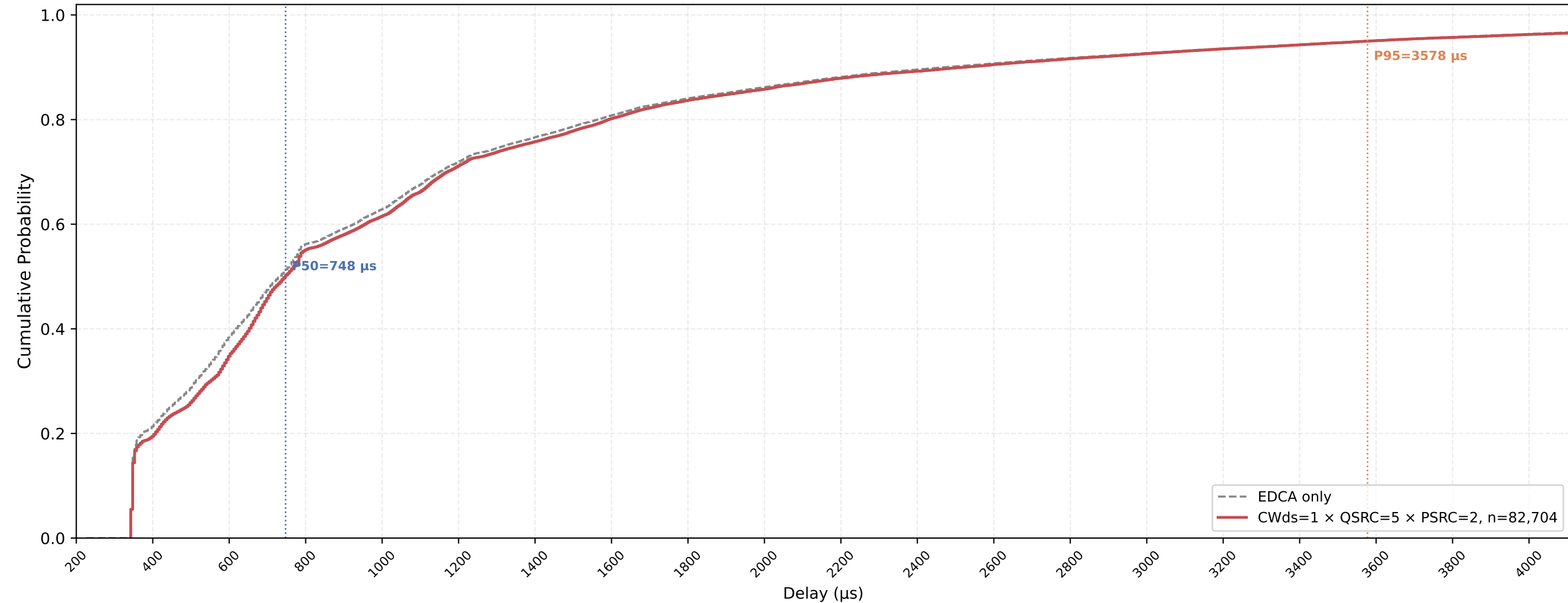
Legacy STA VO Delay CDF — CWds=1 × QSRC=5 × PSRC=2 nSta=30, nPedca=15, 0.5Mbps, avg of 10 runs
