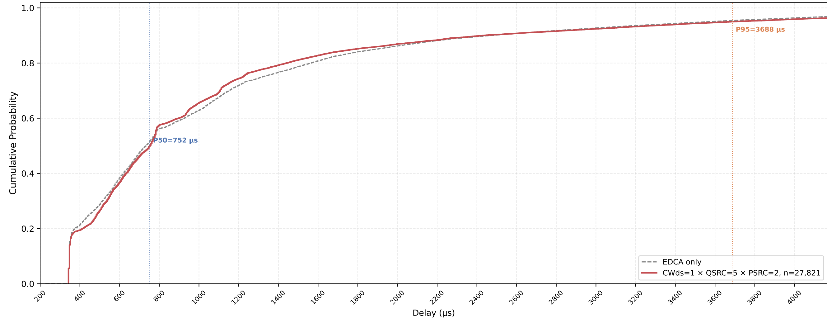
P-EDCA STA VO Delay CDF — CWds=1 × QSRC=5 × PSRC=2 nSta=30, nPedca=5, 0.5Mbps, avg of 10 runs
