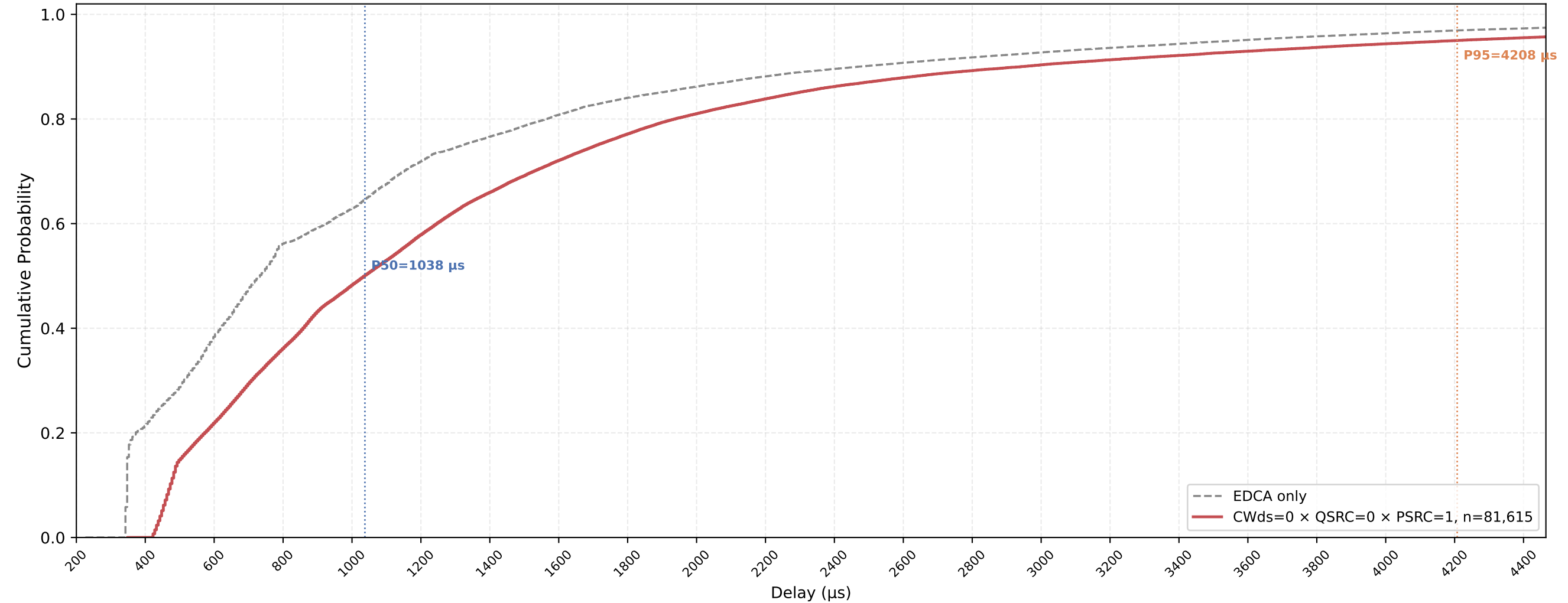
P-EDCA STA VO Delay CDF — CWds=0 × QSRC=0 × PSRC=1 nSta=30, nPedca=15, 0.5Mbps, avg of 10 runs
