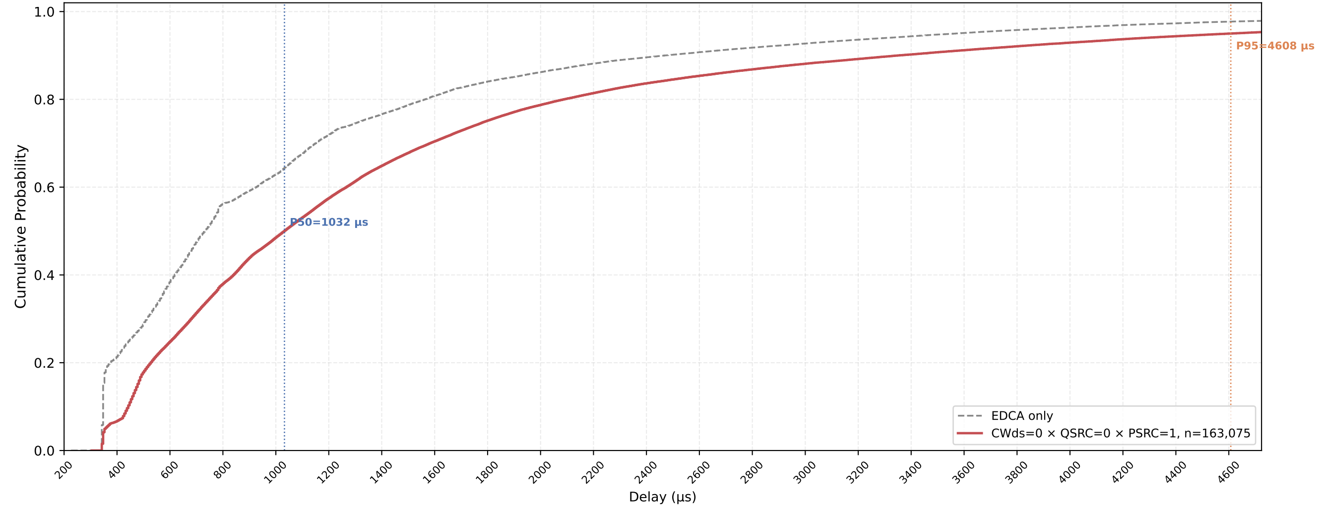
VO (all STAs) Delay CDF — CWds=0 × QSRC=0 × PSRC=1 nSta=30, nPedca=15, 0.5Mbps, avg of 10 runs
