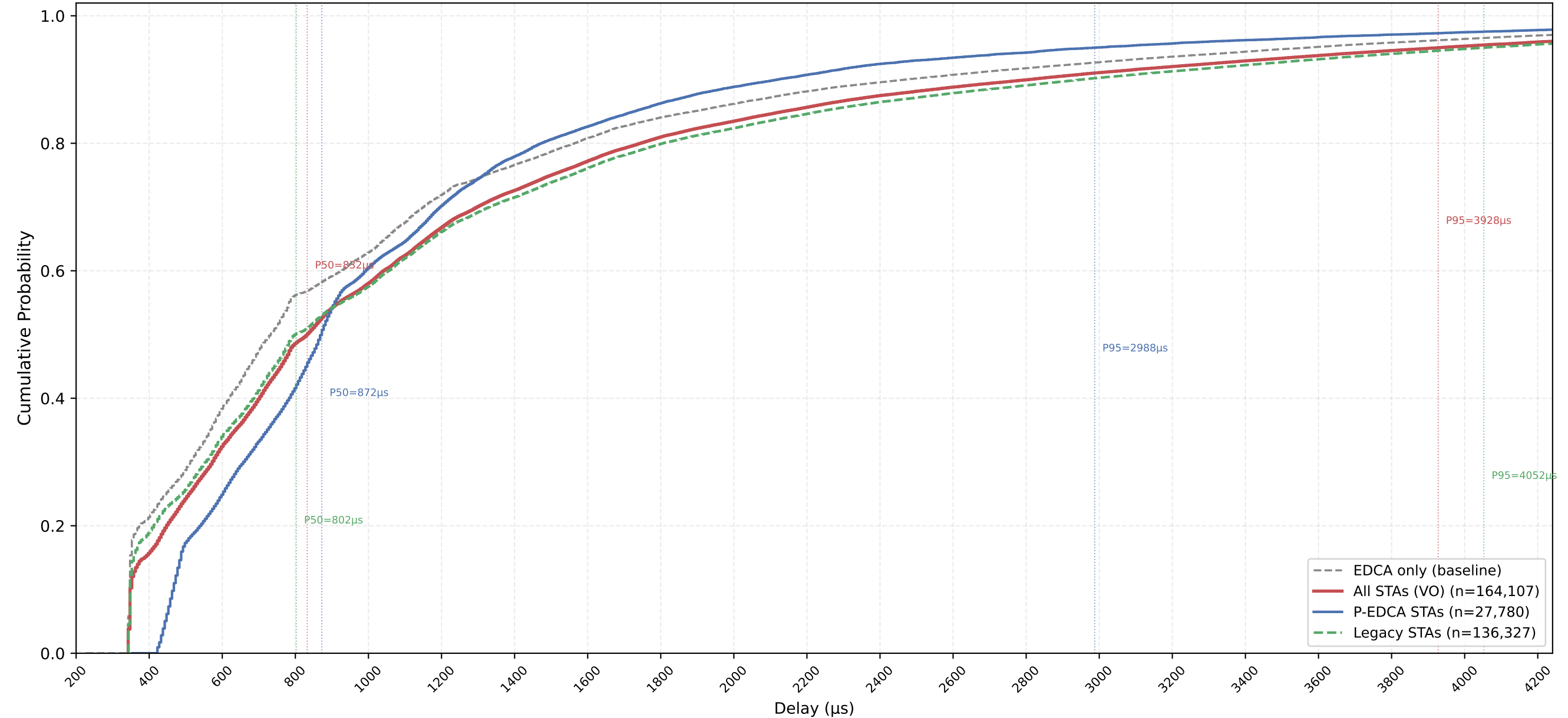
VO Delay CDF — P-EDCA / Legacy / All | CWds=0 × QSRC=0 × PSRC=3 nSta=30, nPedca=5/30, 0.5Mbps, avg of 10 runs
