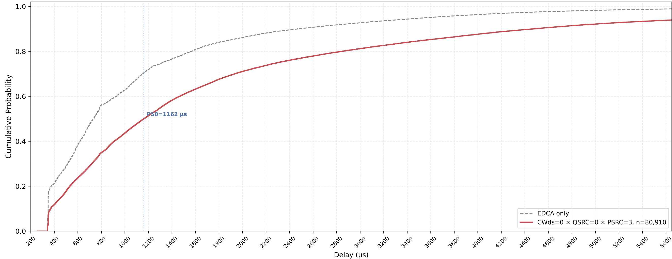
Legacy STA VO Delay CDF — CWds=0 × QSRC=0 × PSRC=3 nSta=30, nPedca=15, 0.5Mbps, avg of 10 runs
