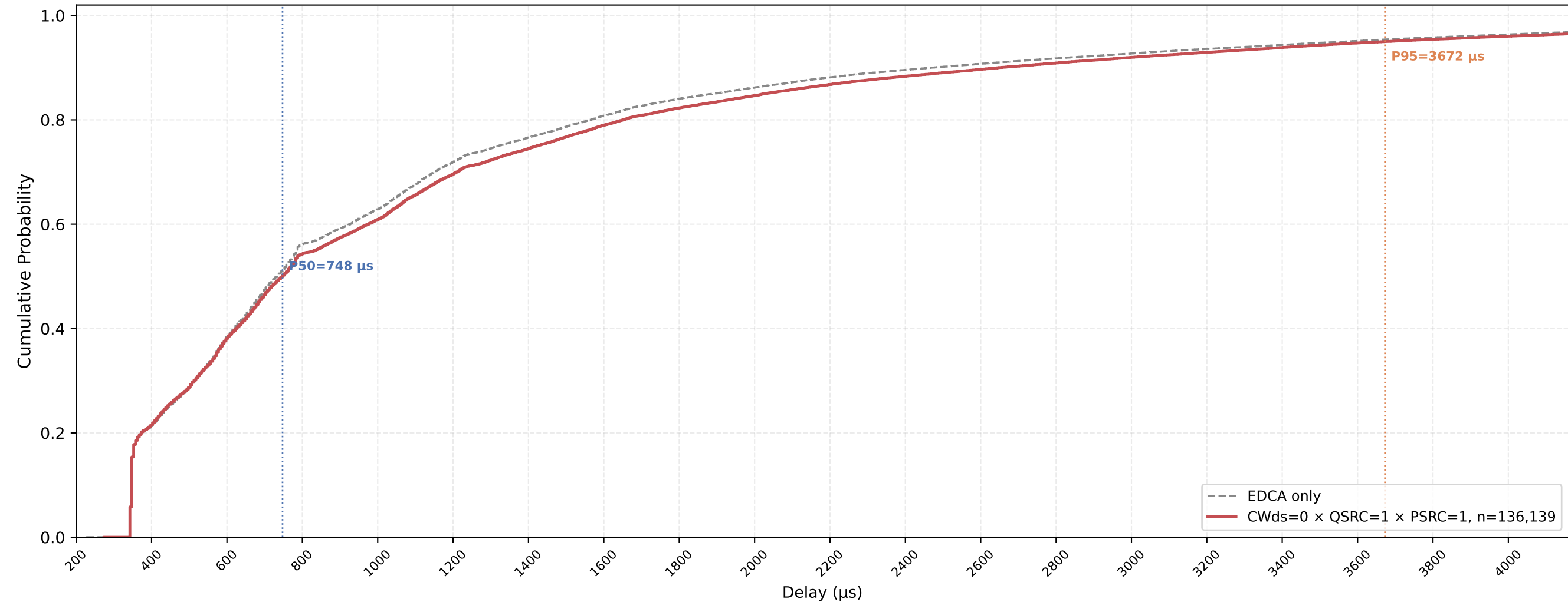
Legacy STA VO Delay CDF — CWds=0 × QSRC=1 × PSRC=1 nSta=30, nPedca=5, 0.5Mbps, avg of 10 runs
