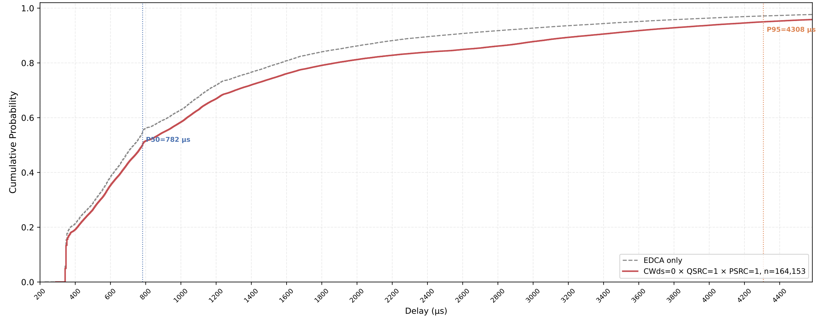
P-EDCA STA VO Delay CDF — CWds=0 × QSRC=1 × PSRC=1 nSta=30, nPedca=30, 0.5Mbps, avg of 10 runs
