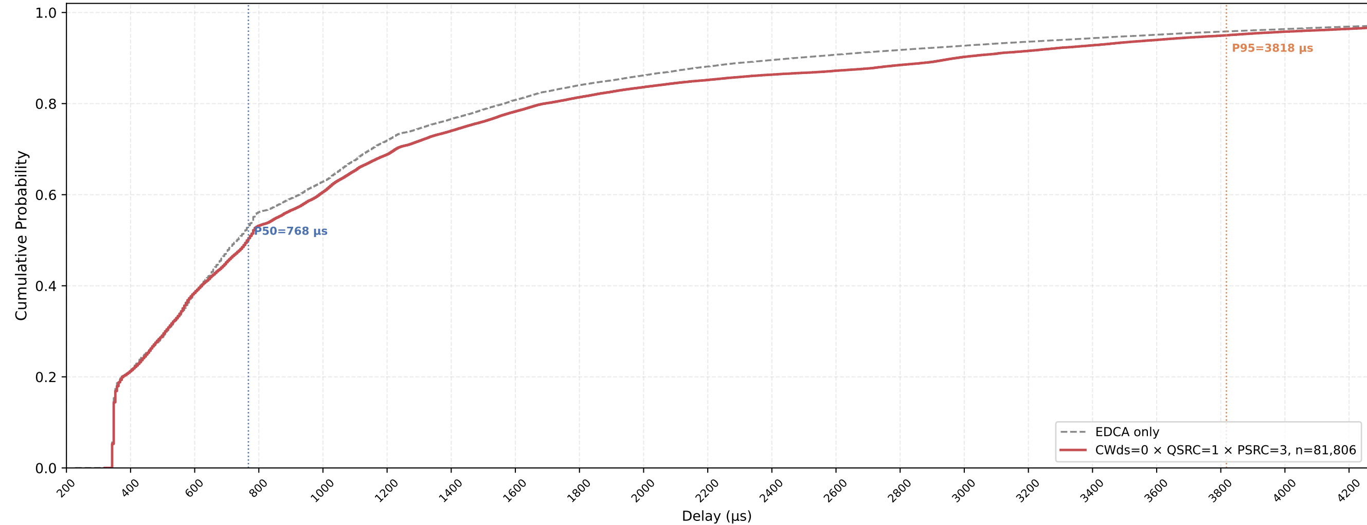
P-EDCA STA VO Delay CDF — CWds=0 × QSRC=1 × PSRC=3 nSta=30, nPedca=15, 0.5Mbps, avg of 10 runs
