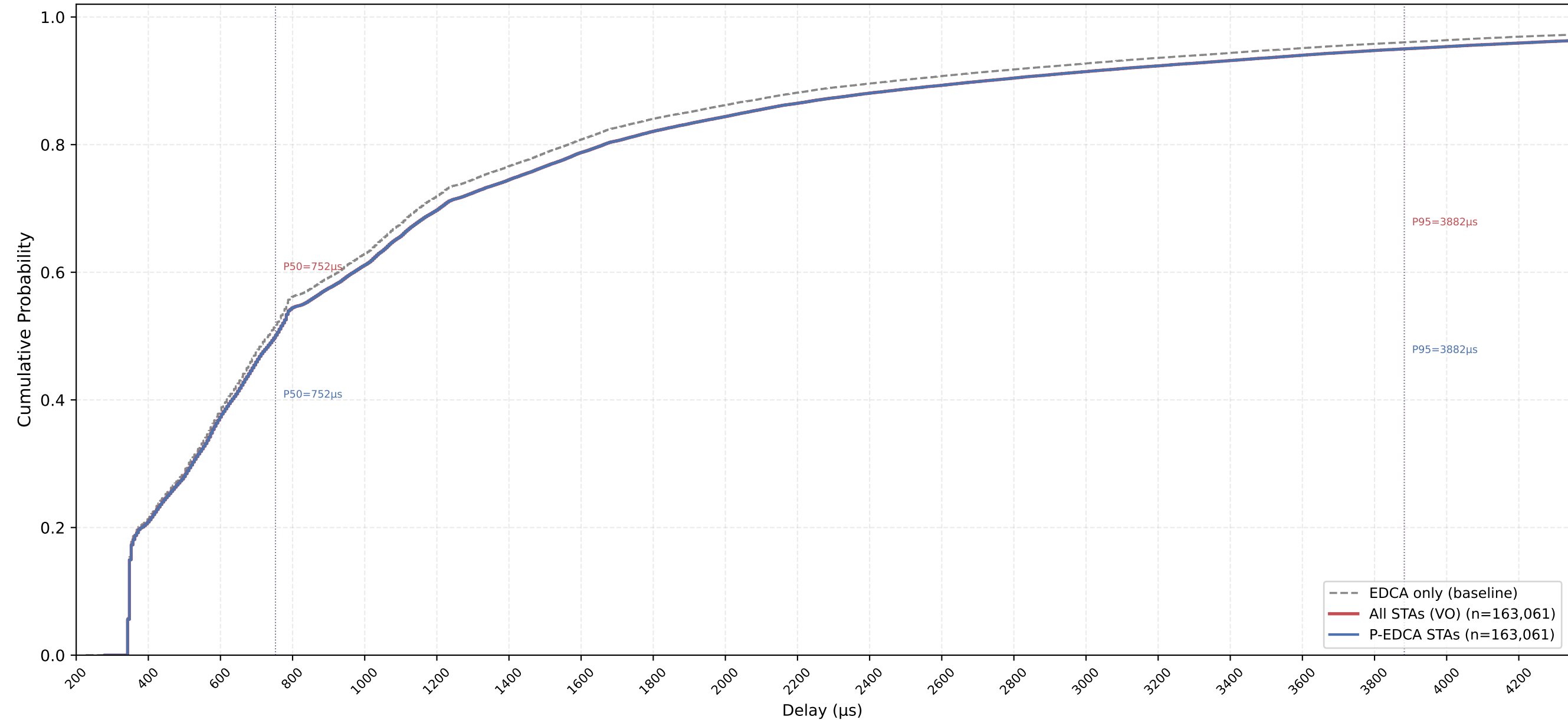
VO Delay CDF — P-EDCA / Legacy / All | CWds=0 × QSRC=2 × PSRC=1 nSta=30, nPedca=30/30, 0.5Mbps, avg of 10 runs
