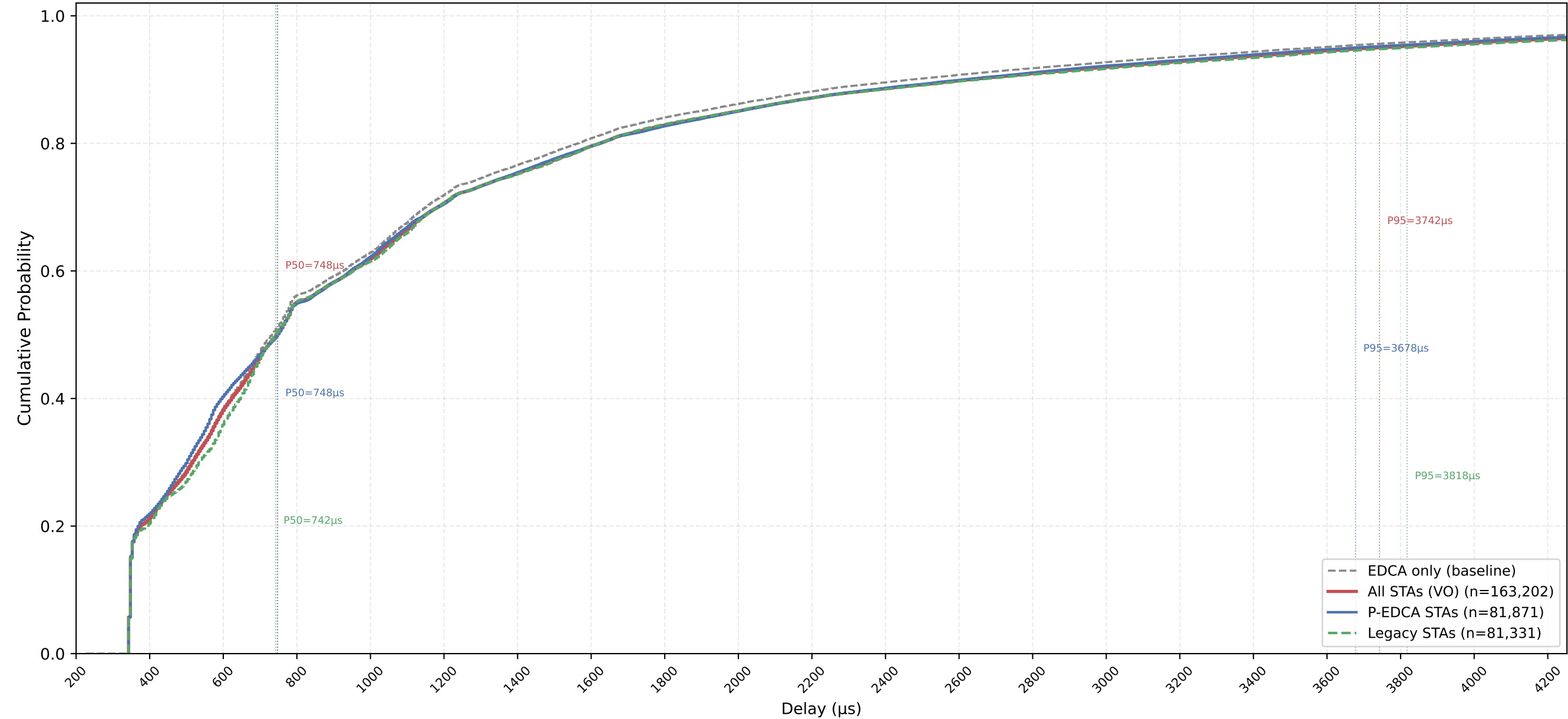
VO Delay CDF — P-EDCA / Legacy / All | CWds=0 × QSRC=2 × PSRC=2 nSta=30, nPedca=15/30, 0.5Mbps, avg of 10 runs
