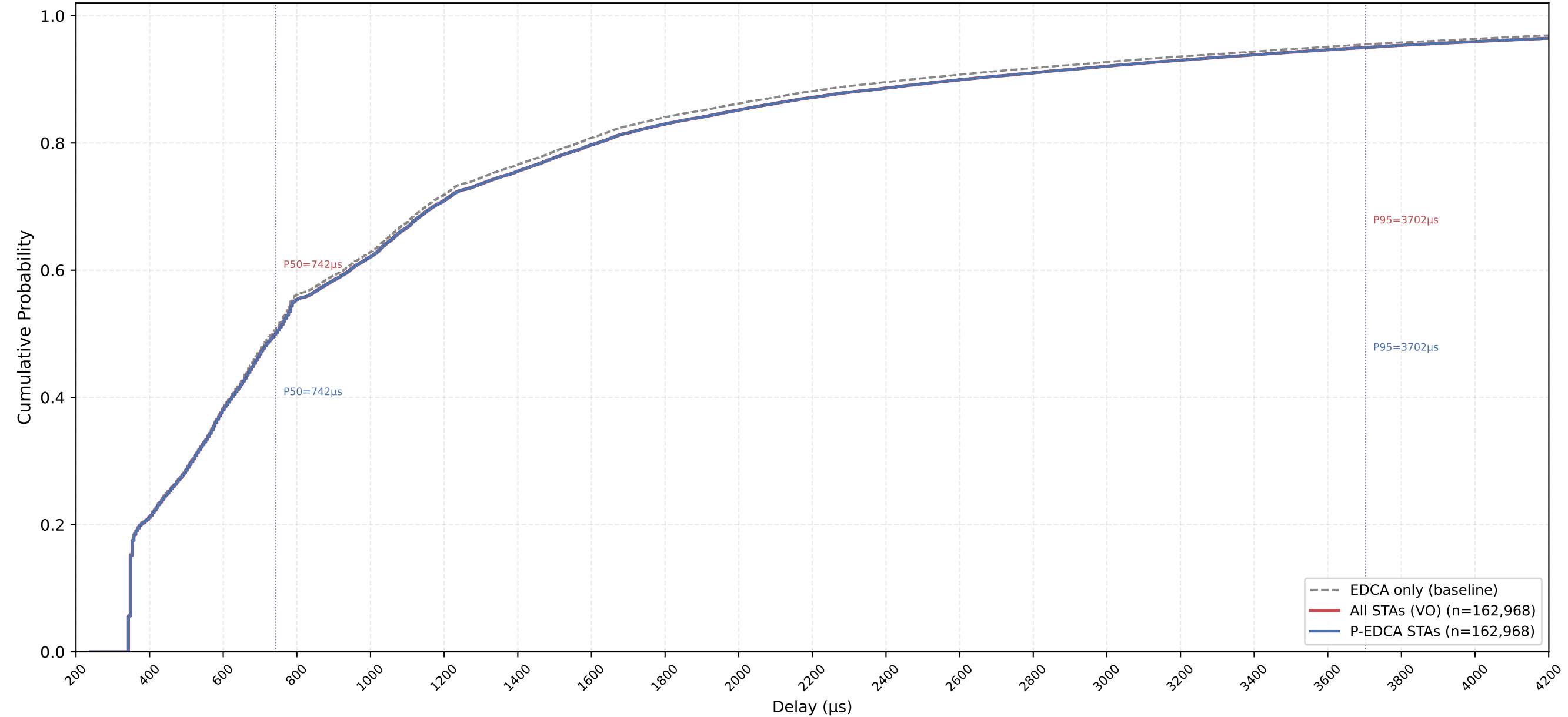
VO Delay CDF — P-EDCA / Legacy / All | CWds=0 × QSRC=3 × PSRC=2 nSta=30, nPedca=30/30, 0.5Mbps, avg of 10 runs
