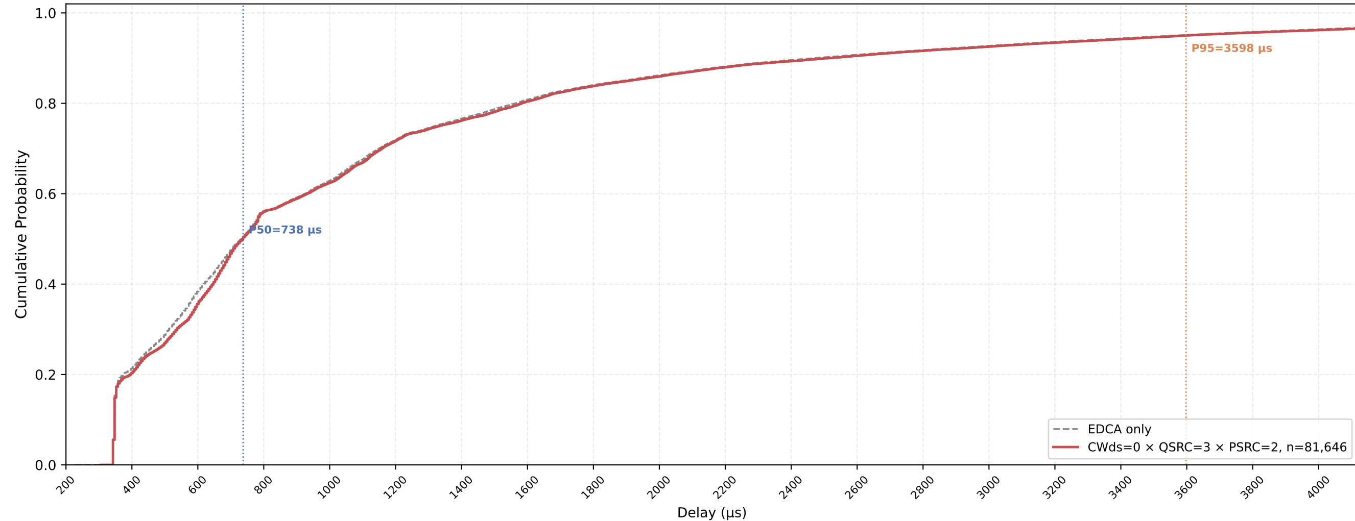
Legacy STA VO Delay CDF — CWds=0 × QSRC=3 × PSRC=2 nSta=30, nPedca=15, 0.5Mbps, avg of 10 runs
