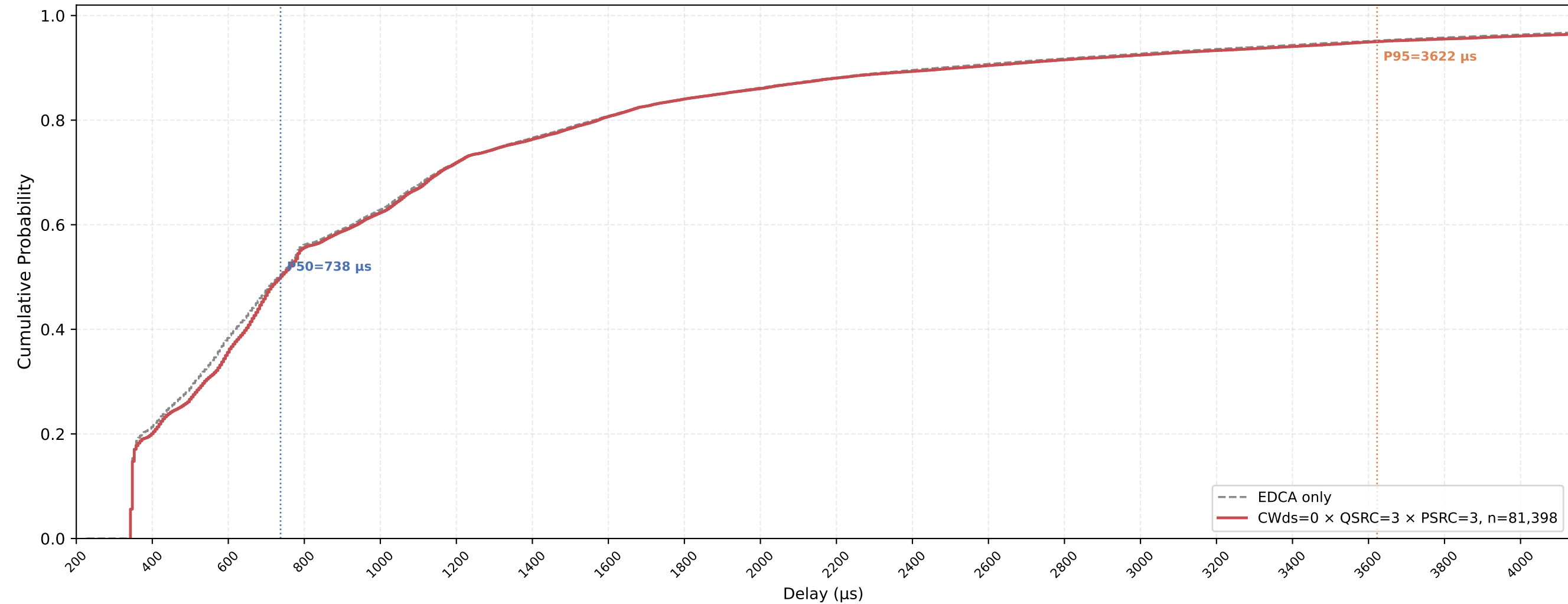
Legacy STA VO Delay CDF — CWds=0 × QSRC=3 × PSRC=3 nSta=30, nPedca=15, 0.5Mbps, avg of 10 runs
