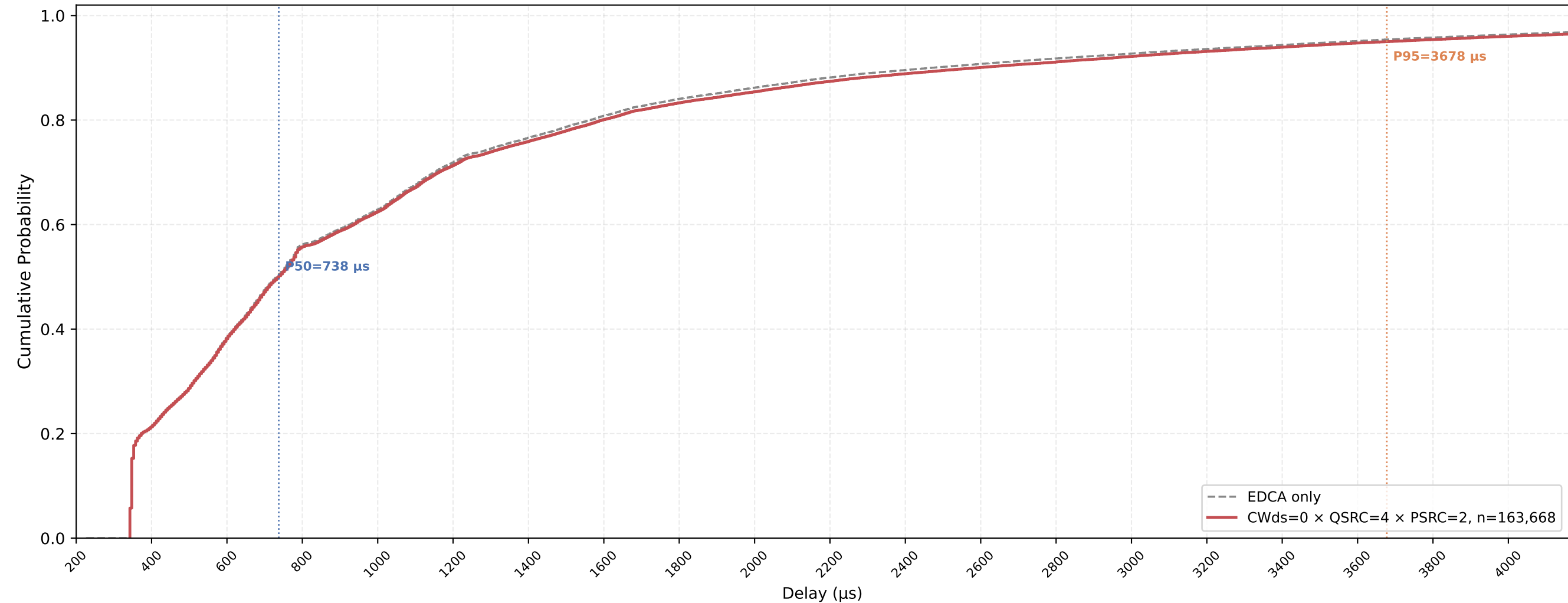
P-EDCA STA VO Delay CDF — CWds=0 × QSRC=4 × PSRC=2 nSta=30, nPedca=30, 0.5Mbps, avg of 10 runs
