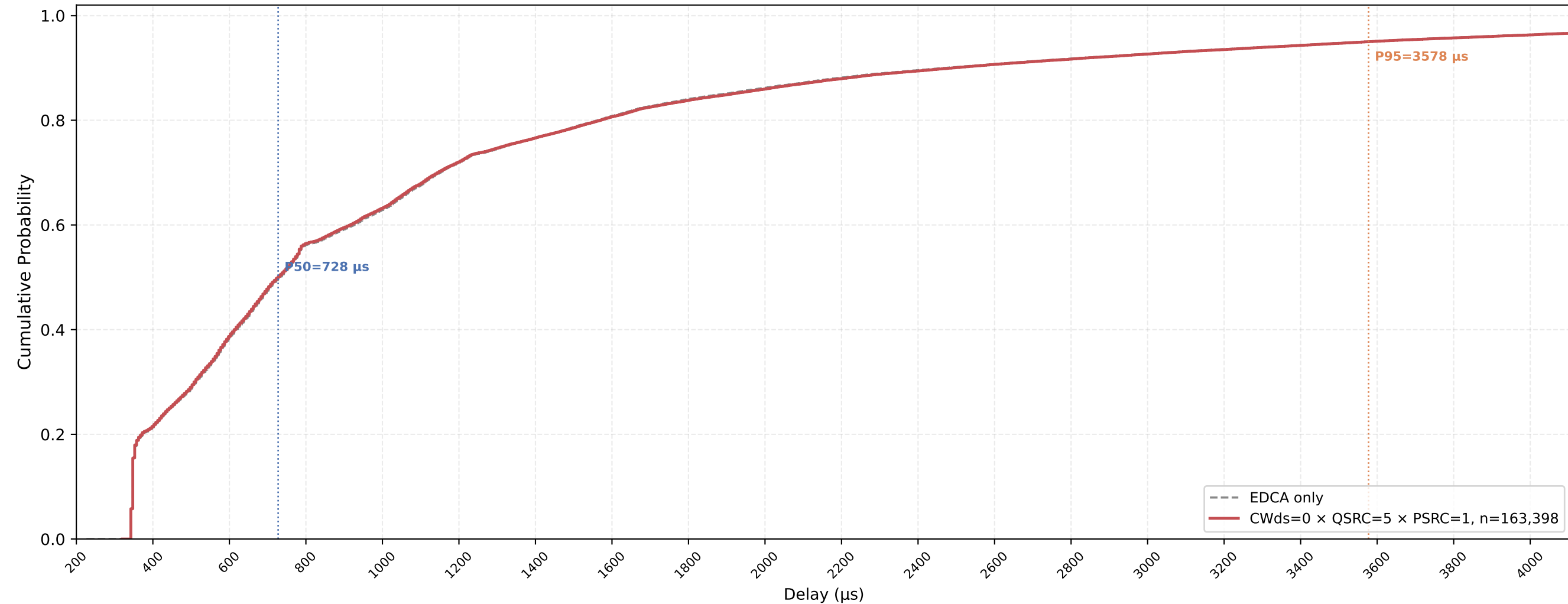
P-EDCA STA VO Delay CDF — CWds=0 × QSRC=5 × PSRC=1 nSta=30, nPedca=30, 0.5Mbps, avg of 10 runs
