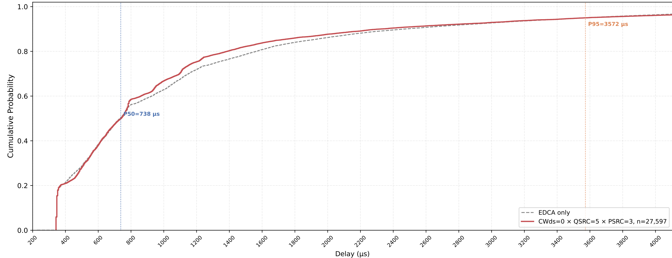
P-EDCA STA VO Delay CDF — CWds=0 × QSRC=5 × PSRC=3 nSta=30, nPedca=5, 0.5Mbps, avg of 10 runs
