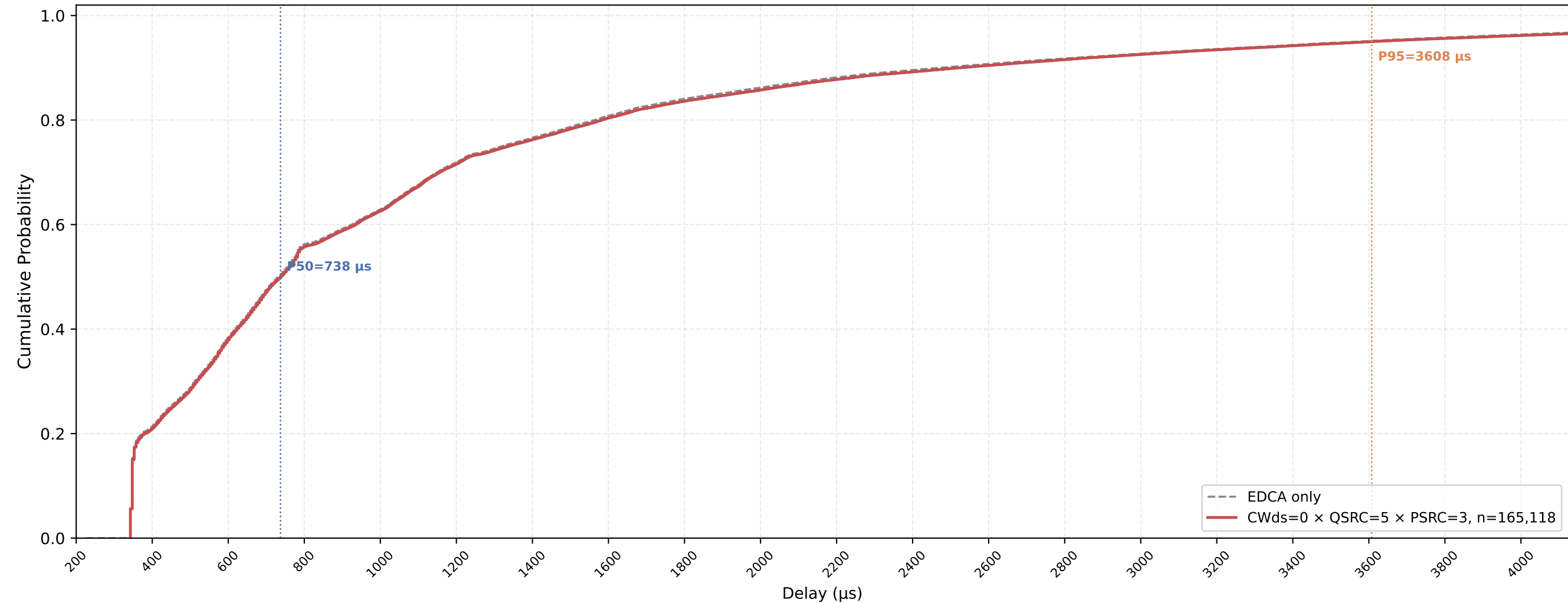
P-EDCA STA VO Delay CDF — CWds=0 × QSRC=5 × PSRC=3 nSta=30, nPedca=30, 0.5Mbps, avg of 10 runs
