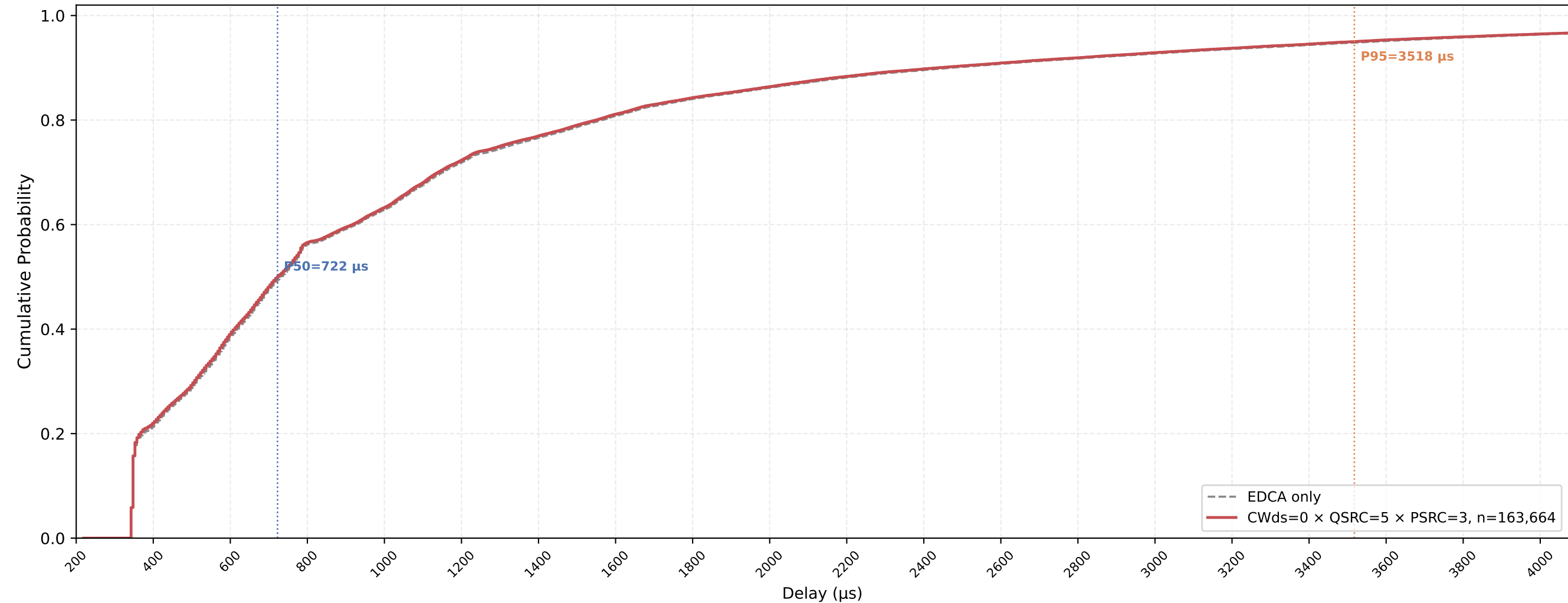
VO (all STAs) Delay CDF — CWds=0 × QSRC=5 × PSRC=3 nSta=30, nPedca=5, 0.5Mbps, avg of 10 runs
