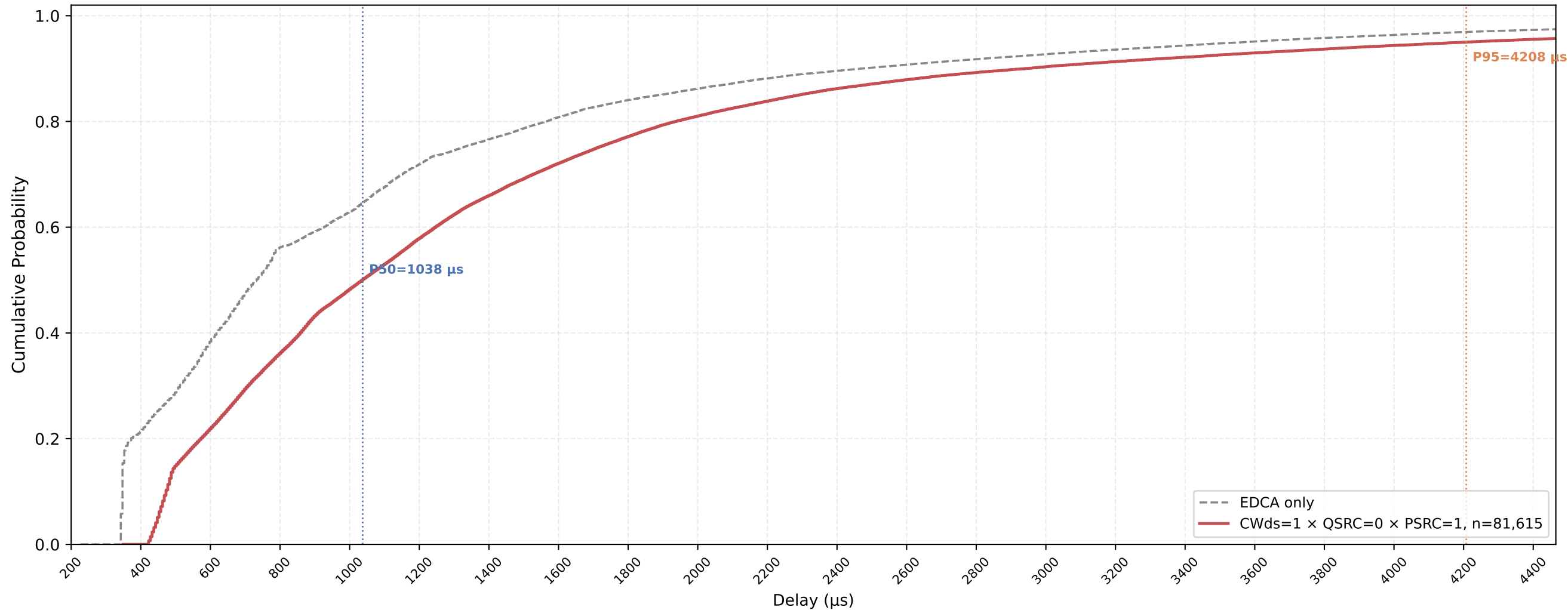
P-EDCA STA VO Delay CDF — CWds=1 × QSRC=0 × PSRC=1 nSta=30, nPedca=15, 0.5Mbps, avg of 10 runs
