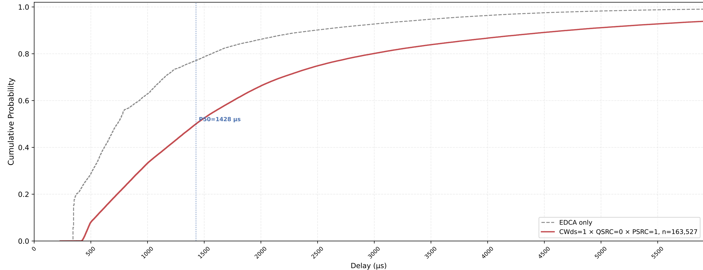
P-EDCA STA VO Delay CDF — CWds=1 × QSRC=0 × PSRC=1 nSta=30, nPedca=30, 0.5Mbps, avg of 10 runs
