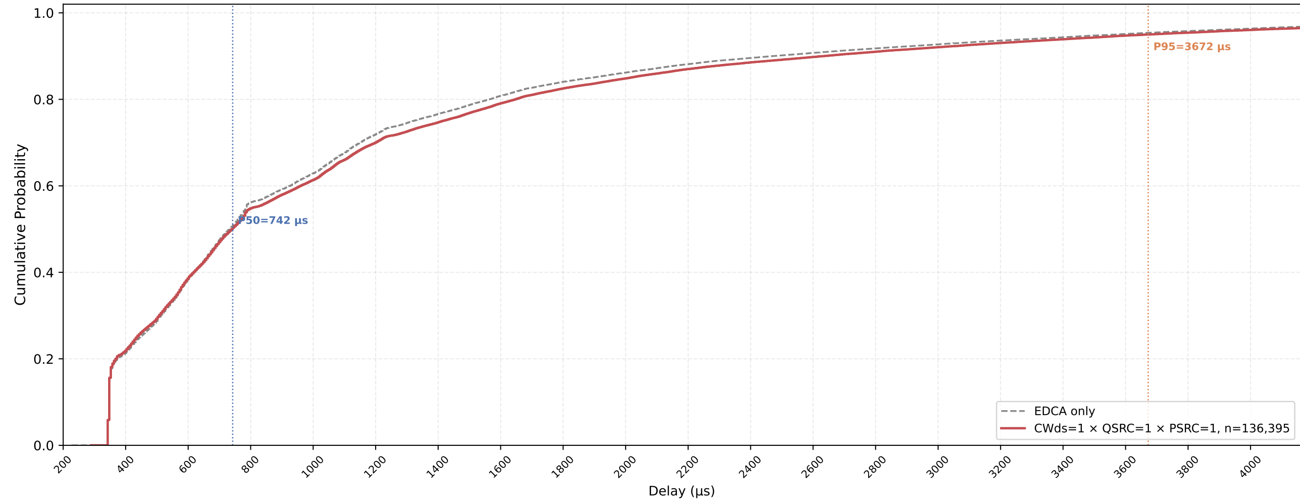
Legacy STA VO Delay CDF — CWds=1 × QSRC=1 × PSRC=1 nSta=30, nPedca=5, 0.5Mbps, avg of 10 runs
