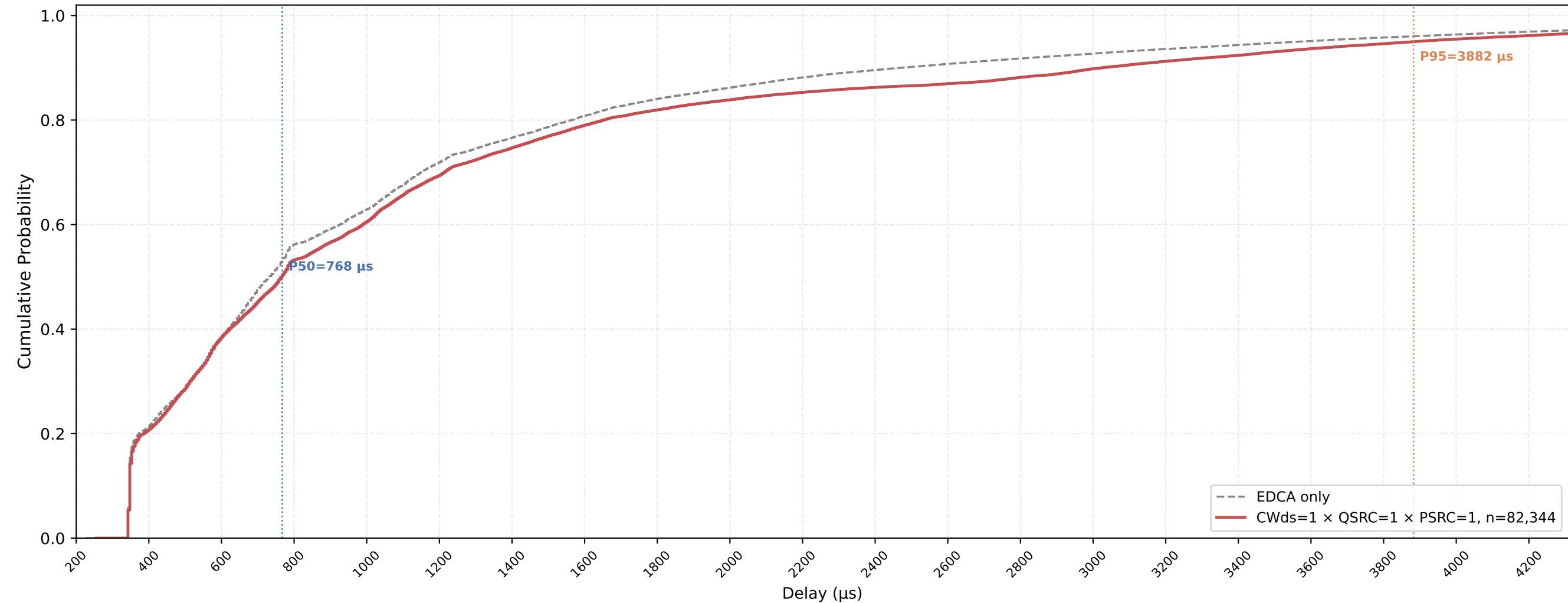
P-EDCA STA VO Delay CDF — CWds=1 × QSRC=1 × PSRC=1 nSta=30, nPedca=15, 0.5Mbps, avg of 10 runs
